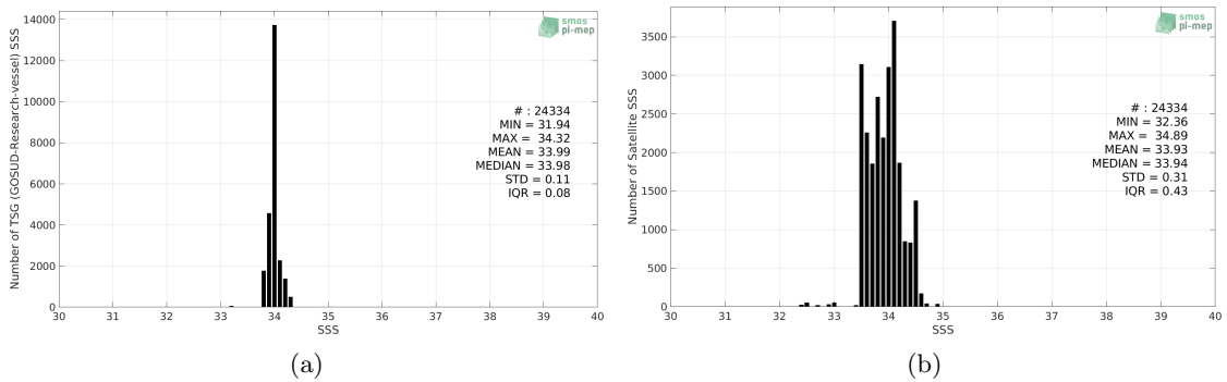
Figure 2: Histograms of SSS from TSG (GOSUD-Research-vessel) (a) and SMOS L4 v2 Weekly (CATDS-CECOS-IFREMER) (b) considering all match-up pairs per bins of 0.1 over the Southern Ocean Pi-MEP region and for the full satellite product period.
