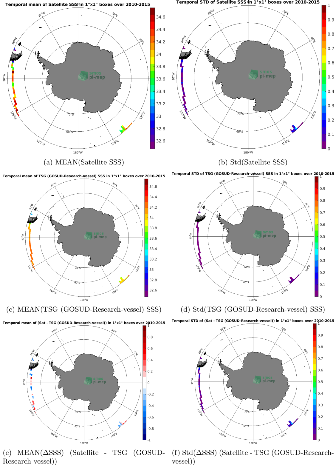
Figure 6: Temporal mean (left) and Std (right) of SSS from SMOS L4 v2 Weekly (CATDS-CECOS-IFREMER) (top), TSG (GOSUD-Research-vessel) (middle), and of \Delta SSS (Satellite - TSG (GOSUD-Research-vessel)). Only match- up pairs are used to generate these maps.
