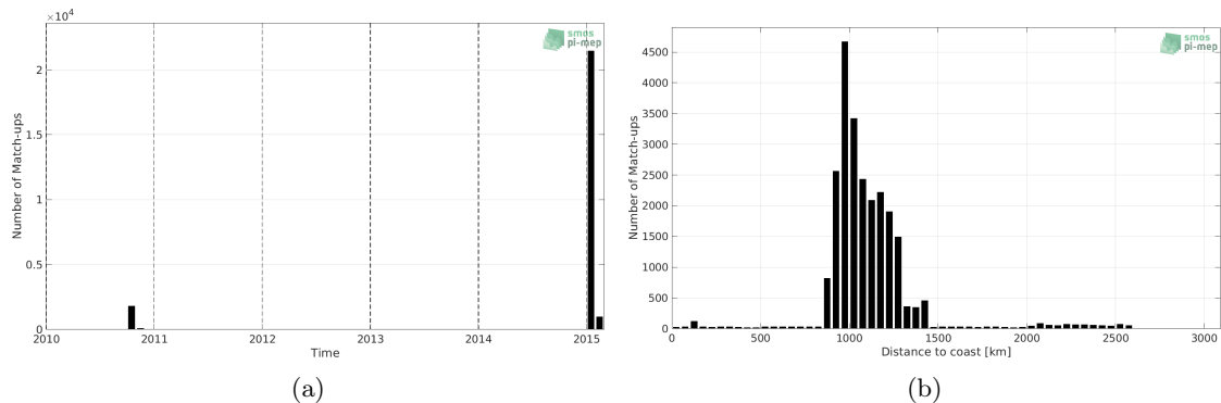
Figure 1: Number of match-ups between TSG (GOSUD-Research-vessel) and SMOS L4 v2 Weekly (CATDS-CECOS-IFREMER) SSS as a function of time (a) and as function of the distance to coast (b) over the Southern Ocean Pi-MEP region and for the full satellite product period.
