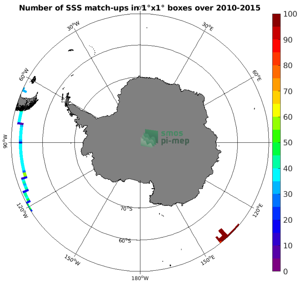
Figure 4: Number of SSS match-ups between TSG (GOSUD-Research-vessel) SSS and the SMOS L4 v2 Weekly (CATDS-CECOS-IFREMER) SSS product for the Southern Ocean Pi-MEP region over 1^\circ \times 1^\circ boxes and for the full satellite product period.
