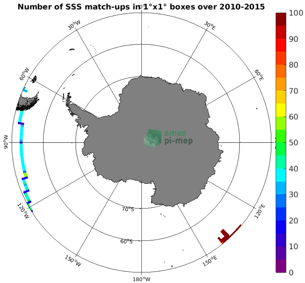
Figure 4: Number of SSS match-ups between TSG (GOSUD-Research-vessel) SSS and the SMOS L4 v2 Weekly (CATDS-CECOS-IFREMER) SSS product for the Southern Ocean Pi-MEP region over 1°x1° boxes and for the full satellite product period.
