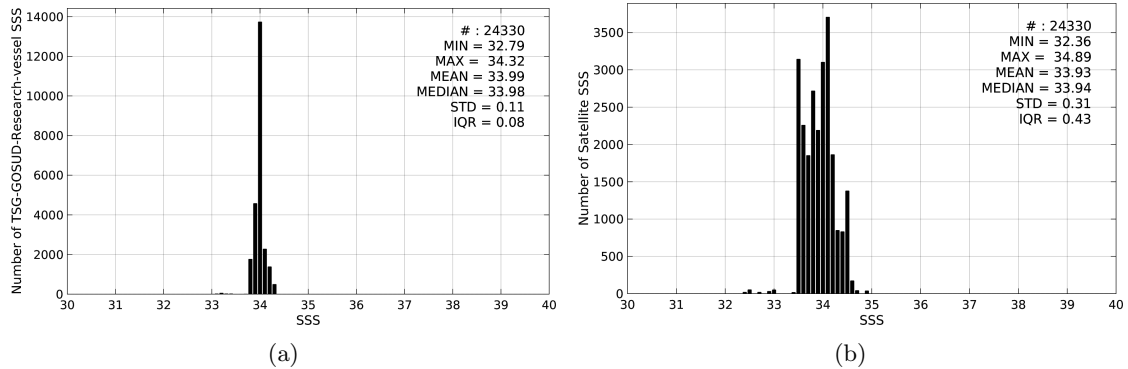
Figure 2: Histograms of SSS from TSG-GOSUD-Research-vessel (a) and SMOS-L4-CATDS-CECOS-IFREMER-V2-WEEKLY-0.5DEG (b) considering all match-up pairs per bins of 0.1 over the Southern Ocean Pi-MEP region and for the full satellite product period.
