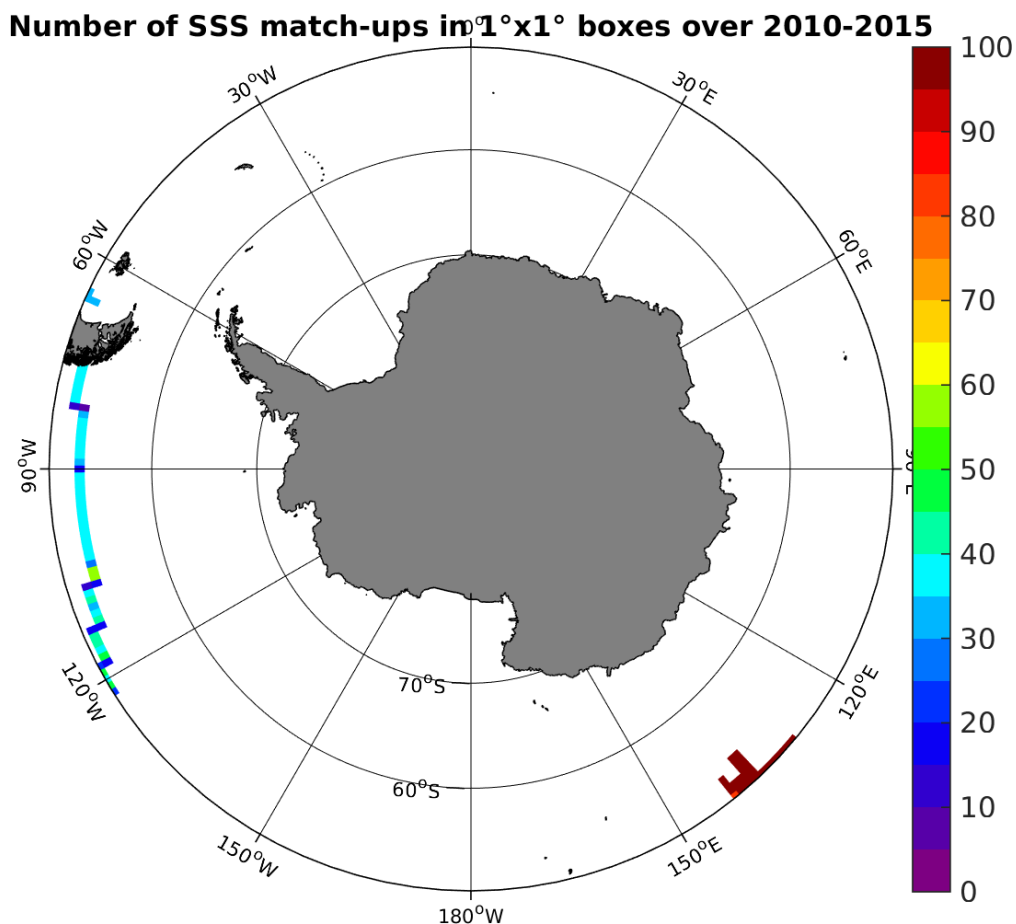
Figure 4: Number of SSS match-ups between TSG-GOSUD-Research-vessel SSS and the SMOS-L4-CATDS-CECOS-IFREMER-V2-WEEKLY-0.5DEG SSS product for the Southern Ocean Pi-MEP region over 1^\circ \times 1^\circ boxes and for the full satellite product period.
