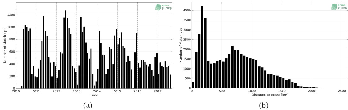
Figure 1: Number of match-ups between Sea mammals and SMOS L4 v2 Weekly (CATDS-CECOS-IFREMER) SSS as a function of time (a) and as function of the distance to coast (b) over the Southern Ocean Pi-MEP region and for the full satellite product period.
