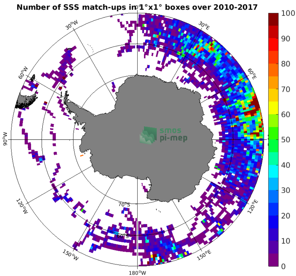
Figure 4: Number of SSS match-ups between Sea mammals SSS and the SMOS L4 v2 Weekly (CATDS-CECOS-IFREMER) SSS product for the Southern Ocean Pi-MEP region over 1^\circ \times 1^\circ boxes and for the full satellite product period.
