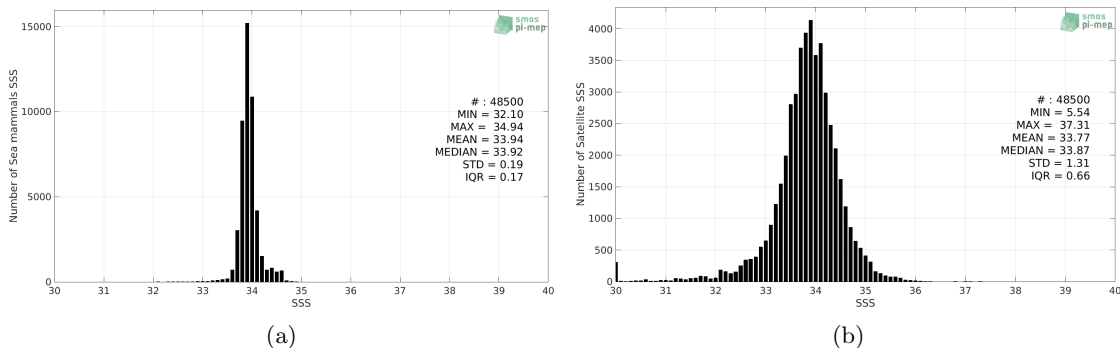
Figure 2: Histograms of SSS from Sea mammals (a) and SMOS L4 v2 Weekly (CATDS-CECOS-IFREMER) (b) considering all match-up pairs per bins of 0.1 over the Southern Ocean Pi-MEP region and for the full satellite product period.
