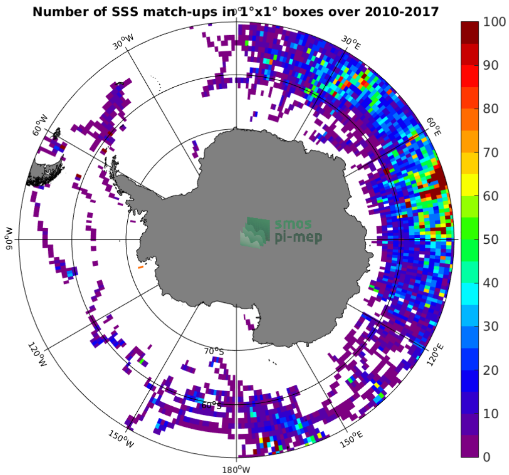
Figure 4: Number of SSS match-ups between Sea mammals SSS and the SMOS-L4-CATDS-CECOS-IFREMER-V2-WEEKLY-0.5DEG SSS product for the Southern Ocean Pi-MEP region over 1^\circ \times 1^\circ boxes and for the full satellite product period.
