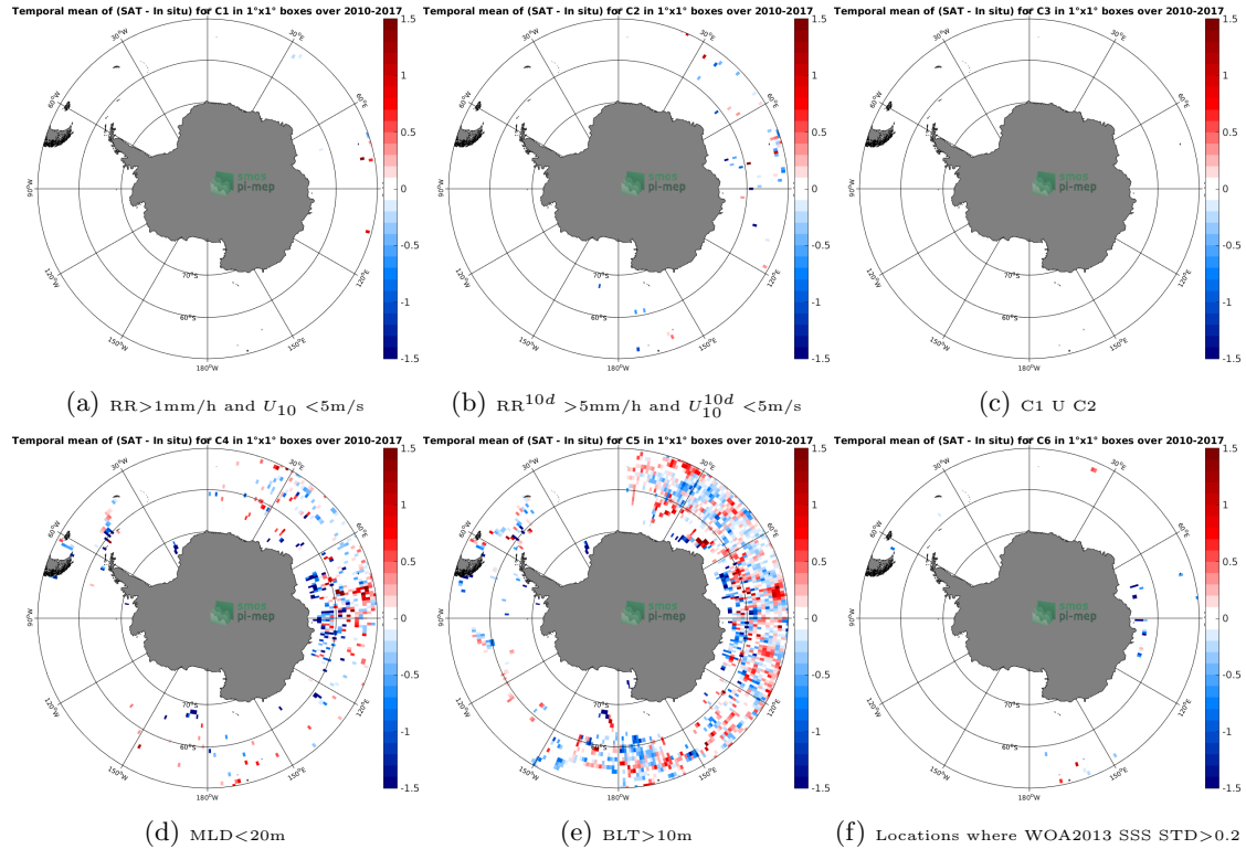
Figure 12: Temporal mean gridded over spatial boxes of size 1^\circ \times 1^\circ of \Delta\text{SSS} (SMOS-L4-CATDS-CECOS-IFREMER-V2-WEEKLY-0.5DEG - Sea mammals) for 6 different subdatasets corresponding to: \text{RR} > 1\text{mm/h} and U_{10} < 5\text{m/s} (a), \text{RR}^{10d} > 5\text{mm/h} and U_{10}^{10d} < 5\text{m/s} (b), C1 U C2 (c), \text{MLD} < 20\text{m} (d), \text{BLT} > 10\text{m} (e), Locations where WOA2013 SSS \text{STD} > 0.2 (f).
