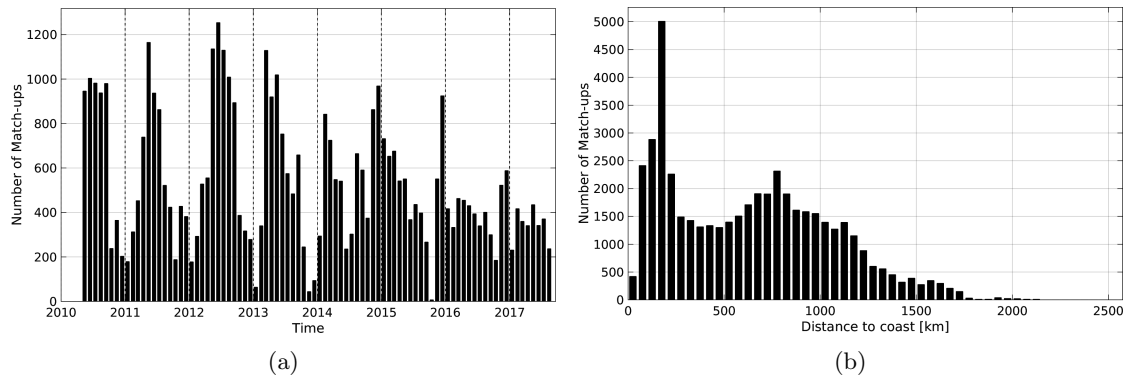
Figure 1: Number of match-ups between Sea mammals and SMOS-L4-CATDS-CECOS-IFREMER-V2-WEEKLY-0.5DEG SSS as a function of time (a) and as function of the distance to coast (b) over the Southern Ocean Pi-MEP region and for the full satellite product period.
