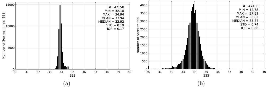
Figure 2: Histograms of SSS from Sea mammals (a) and SMOS-L4-CATDS-CECOS-IFREMER-V2-WEEKLY-0.5DEG (b) considering all match-up pairs per bins of 0.1 over the Southern Ocean Pi-MEP region and for the full satellite product period.
