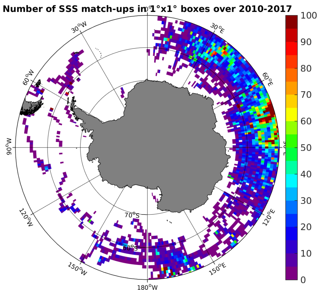
Figure 4: Number of SSS match-ups between Sea mammals SSS and the SMOS-L4-CATDS-CECOS-IFREMER-V2-WEEKLY-0.5DEG SSS product for the Southern Ocean Pi-MEP region over 1°x1° boxes and for the full satellite product period.
