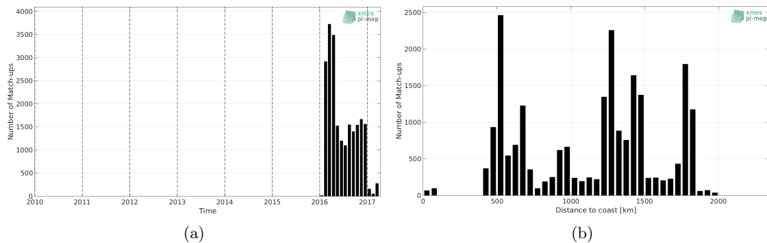
Figure 1: Number of match-ups between Surface drifters and SMOS-L4-CATDS-CECOS-IFREMER-V2-WEEKLY-0.5DEG SSS as a function of time (a) and as function of the distance to coast (b) over the Southern Ocean Pi-MEP region and for the full satellite product period.
