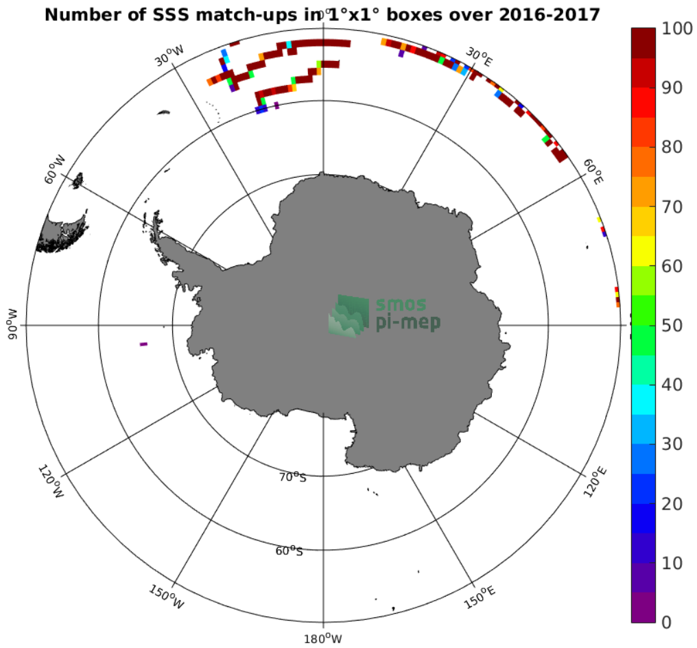
Figure 3: Number of SSS match-ups between Surface drifters SSS and the SMOS-L4-CATDS-CECOS-IFREMER-V2-WEEKLY-0.5DEG SSS product for the Southern Ocean Pi-MEP region over 1°x1° boxes and for the full satellite product period.
