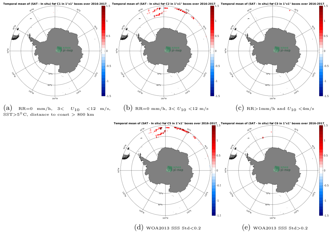
Figure 11: Temporal mean gridded over spatial boxes of size 1^\circ \times 1^\circ of \Delta SSS (SMOS-L4-CATDS-CECOS-IFREMER-V2-WEEKLY-0.5DEG - Surface drifters) for 5 different subdatasets corresponding to:RR=0 mm/h, 3 < U_{10} < 12 m/s, SST >5^\circ C, distance to coast > 800 km (a), RR=0 mm/h, 3 < U_{10} < 12 m/s (b), RR >1 mm/h and U_{10} < 4 m/s (c), WOA2013 SSS Std <0.2 (d), WOA2013 SSS Std >0.2 (e).
