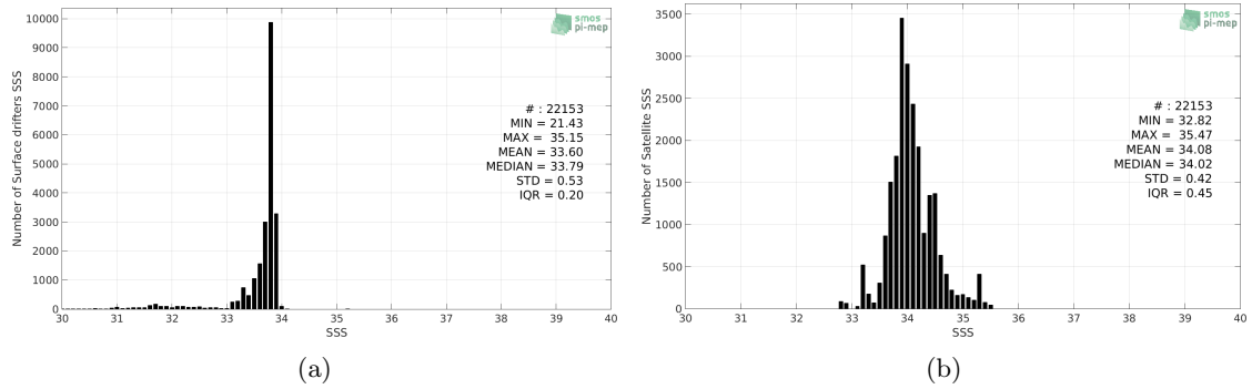
Figure 2: Histograms of SSS from Surface drifters (a) and SMOS-L4-CATDS-CECOS-IFREMER-V2-WEEKLY-0.5DEG (b) considering all match-up pairs per bins of 0.1 over the Southern Ocean Pi-MEP region and for the full satellite product period.
