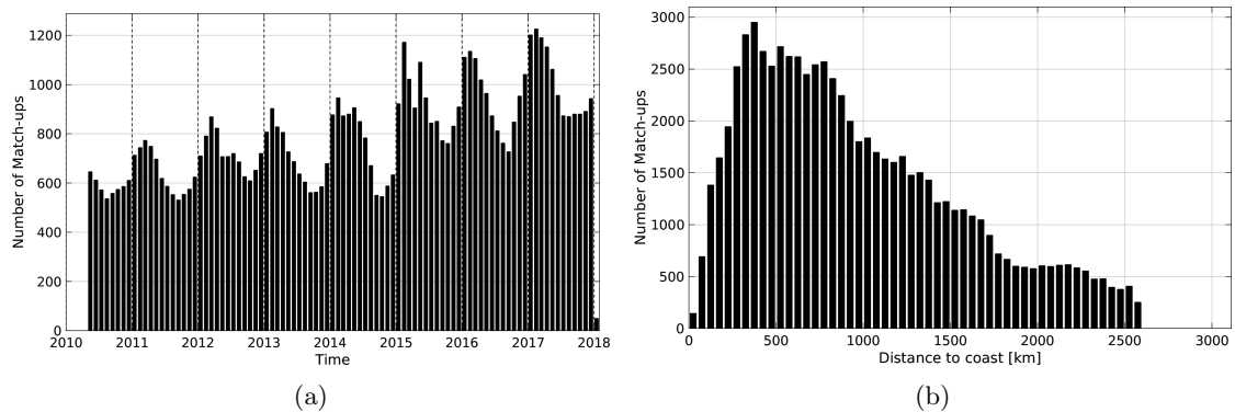
Figure 1: Number of match-ups between Argo and SMOS-L4-CATDS-CECOS-IFREMER-V2-WEEKLY-0.5DEG SSS as a function of time (a) and as function of the distance to coast (b) over the Southern Ocean Pi-MEP region and for the full satellite product period.
