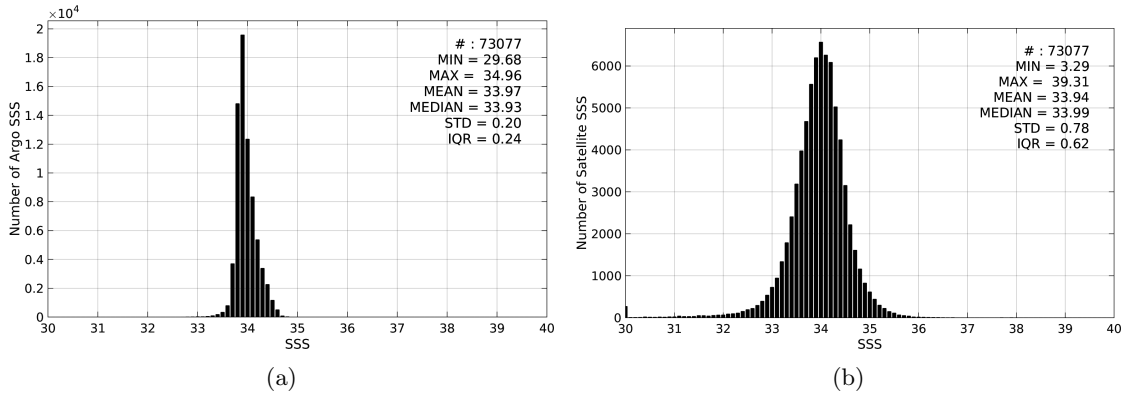
Figure 2: Histograms of SSS from Argo (a) and SMOS-L4-CATDS-CECOS-IFREMER-V2-WEEKLY-0.5DEG (b) considering all match-up pairs per bins of 0.1 over the Southern Ocean Pi-MEP region and for the full satellite product period.
