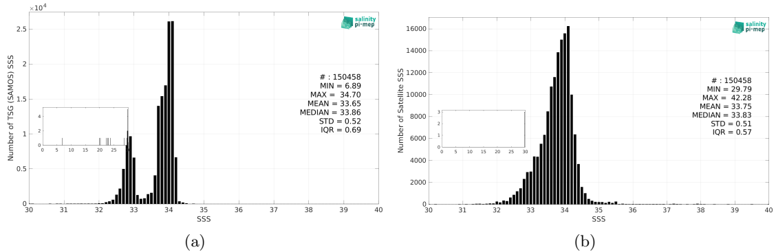
Figure 3: Histograms of SSS from TSG (SAMOS) (a) and SMOS SSS L4 v2 - Daily (BEC) (b) considering all match-up pairs per bins of 0.1 over the Southern Ocean Pi-MEP region and for the full satellite product period.
