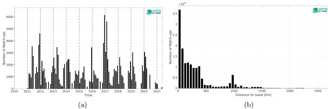
Figure 2: Number of match-ups between TSG (SAMOS) and SMOS SSS L4 v2 - Daily (BEC) SSS as a function of time (a) and as function of the distance to coast (b) over the Southern Ocean Pi-MEP region and for the full satellite product period.
