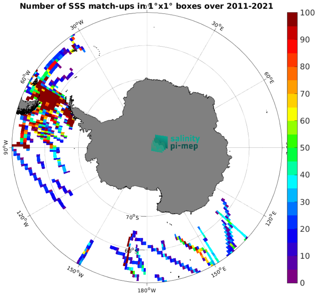
Figure 5: Number of SSS match-ups between TSG (SAMOS) SSS and the SMOS SSS L4 v2 - Daily (BEC) SSS product for the Southern Ocean Pi-MEP region over 1^\circ \times 1^\circ boxes and for the full satellite product period.
