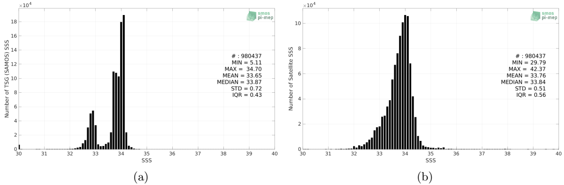
Figure 2: Histograms of SSS from TSG (SAMOS) (a) and SMOS SSS L4 v2 - Daily (BEC) (b) considering all match-up pairs per bins of 0.1 over the Southern Ocean Pi-MEP region and for the full satellite product period.
