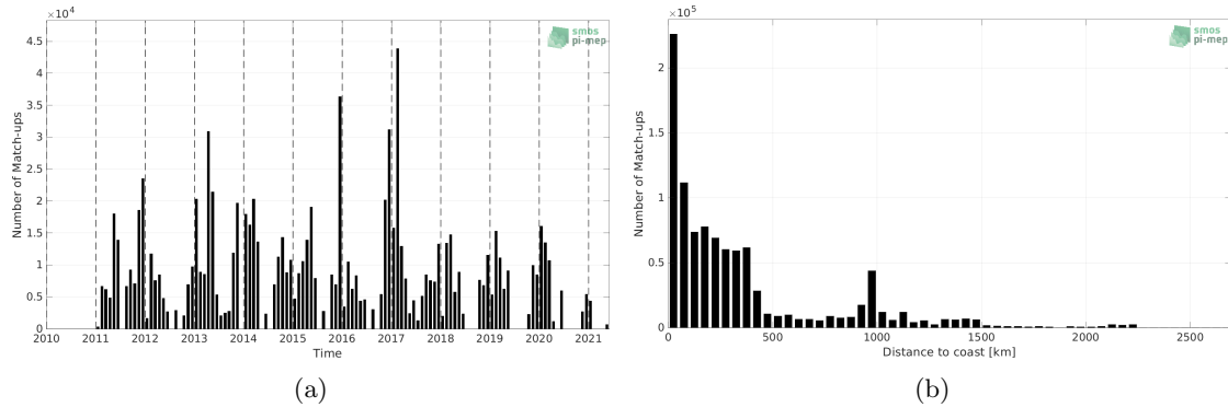
Figure 1: Number of match-ups between TSG (SAMOS) and SMOS SSS L4 v2 - Daily (BEC) SSS as a function of time (a) and as function of the distance to coast (b) over the Southern Ocean Pi-MEP region and for the full satellite product period.
