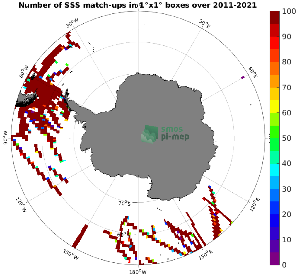
Figure 4: Number of SSS match-ups between TSG (SAMOS) SSS and the SMOS SSS L4 v2 - Daily (BEC) SSS product for the Southern Ocean Pi-MEP region over 1^\circ \times 1^\circ boxes and for the full satellite product period.
