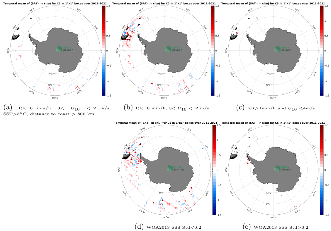
Figure 12: Temporal mean gridded over spatial boxes of size 1^{\circ}\times 1^{\circ} of \Delta\text{SSS} (SMOS SSS L4 v2 - Daily (BEC) - TSG (SAMOS)) for 5 different subdatasets corresponding to:RR=0 mm/h, 3 < U_{10} < 12 m/s, SST >5^{\circ}\text{C} , distance to coast > 800 km (a), RR=0 mm/h, 3 < U_{10} < 12 m/s (b), RR >1 mm/h and U_{10} < 4 m/s (c), WOA2013 SSS Std <0.2 (d), WOA2013 SSS Std >0.2 (e).
