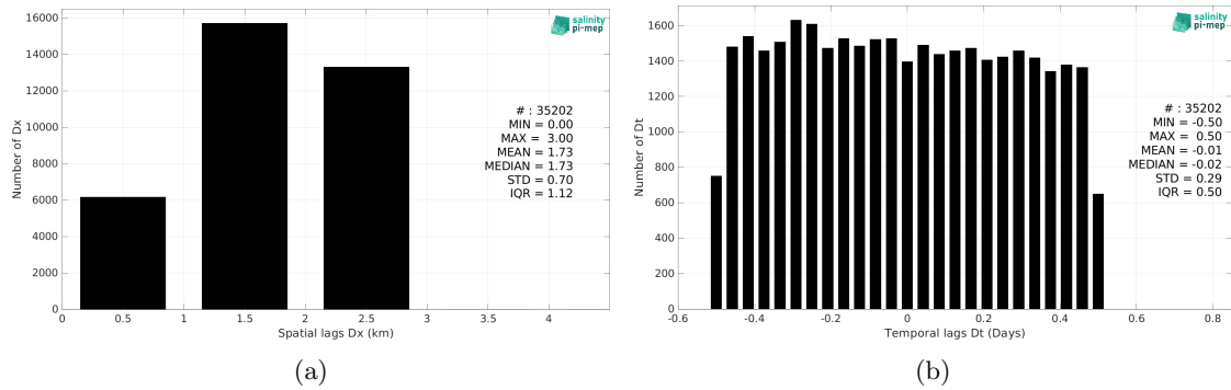
Figure 6: Histograms of the spatial (a) and temporal (b) lags between the location/time of the TSG (Polarstern) measurement and the date of the corresponding SMOS SSS L4 v2 - Daily (BEC) SSS pixel.
