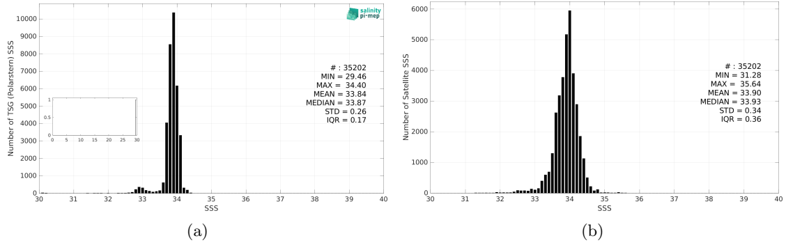
Figure 3: Histograms of SSS from TSG (Polarstern) (a) and SMOS SSS L4 v2 - Daily (BEC) (b) considering all match-up pairs per bins of 0.1 over the Southern Ocean Pi-MEP region and for the full satellite product period.
