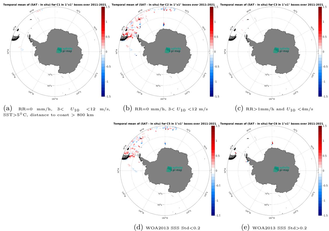
Figure 14: Temporal mean gridded over spatial boxes of size 1^\circ \times 1^\circ of \Delta SSS (SMOS SSS L4 v2 - Daily (BEC) - TSG (Polarstern)) for 5 different subdatasets corresponding to:RR=0 mm/h, 3 < U_{10} < 12 m/s, SST >5^\circ\text{C} , distance to coast > 800 km (a), RR=0 mm/h, 3 < U_{10} < 12 m/s (b), RR >1 mm/h and U_{10} < 4 m/s (c), WOA2013 SSS Std <0.2 (d), WOA2013 SSS Std >0.2 (e).
