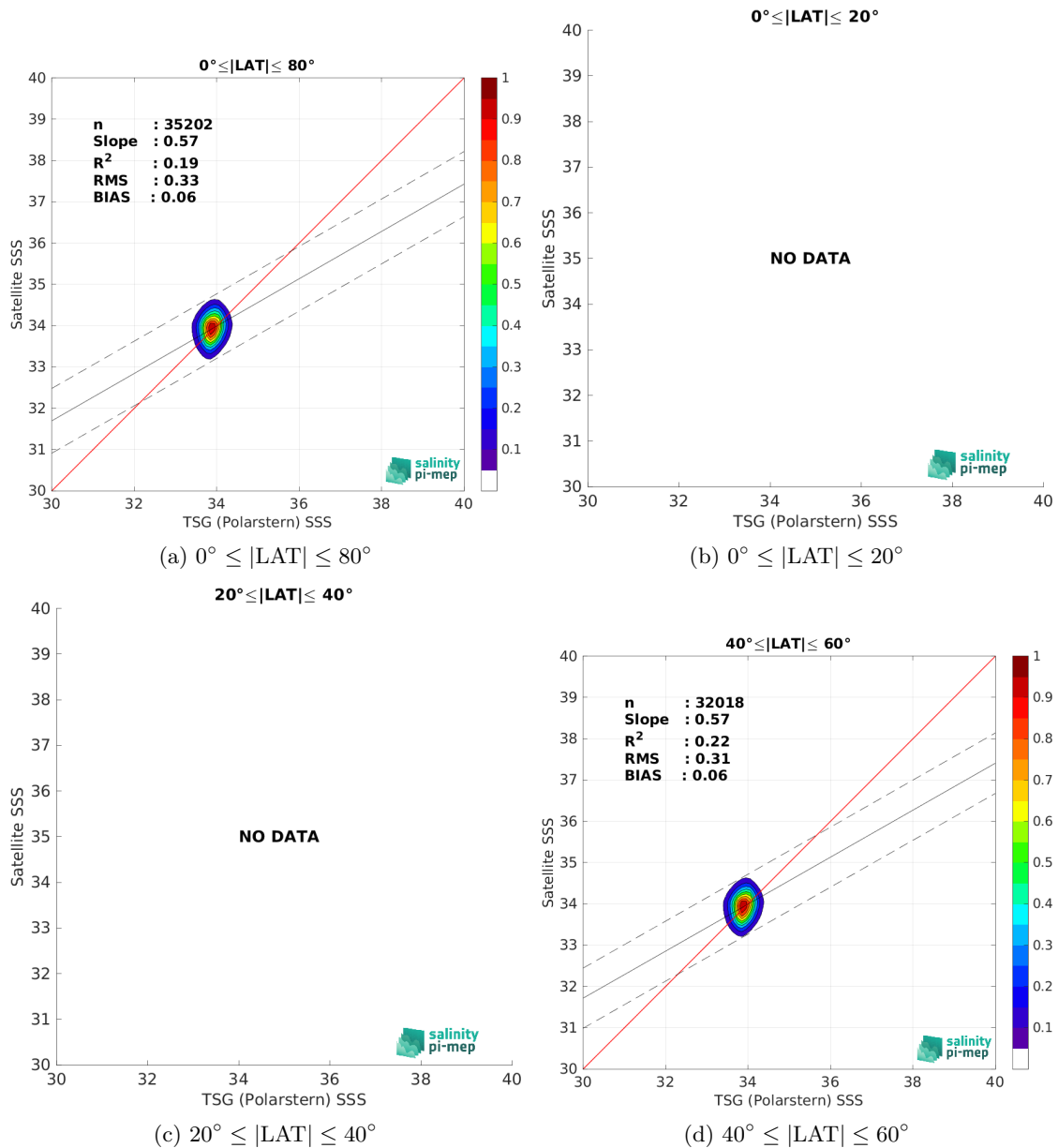
Figure 10: Contour maps of the concentration of SMOS SSS L4 v2 - Daily (BEC) SSS (y-axis) versus TSG (Polarstern) SSS (x-axis) at match-up pairs for different latitude bands. For each plot, the red line shows x=y . The black thin and dashed lines indicate a linear fit through the data cloud and the \pm 95\% confidence levels, respectively. The number match-up pairs n , the slope and R^2 coefficient of the linear fit, the root mean square (RMS) and the mean bias between satellite and in situ data are indicated for each latitude band in each plots.
