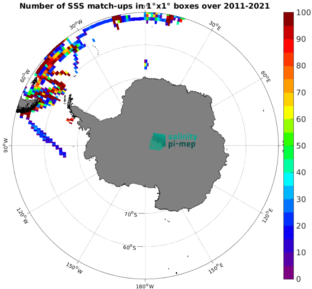
Figure 5: Number of SSS match-ups between TSG (Polarstern) SSS and the SMOS SSS L4 v2 - Daily (BEC) SSS product for the Southern Ocean Pi-MEP region over 1^\circ \times 1^\circ boxes and for the full satellite product period.
