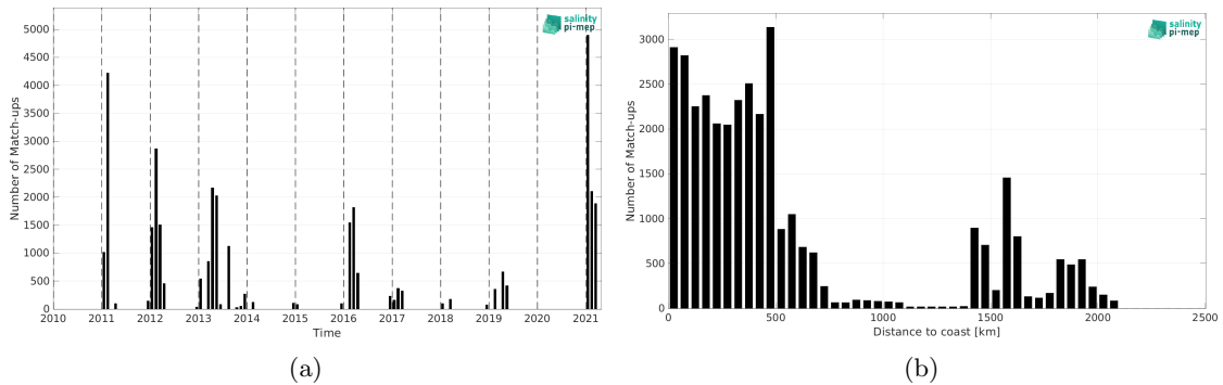
Figure 2: Number of match-ups between TSG (Polarstern) and SMOS SSS L4 v2 - Daily (BEC) SSS as a function of time (a) and as function of the distance to coast (b) over the Southern Ocean Pi-MEP region and for the full satellite product period.
