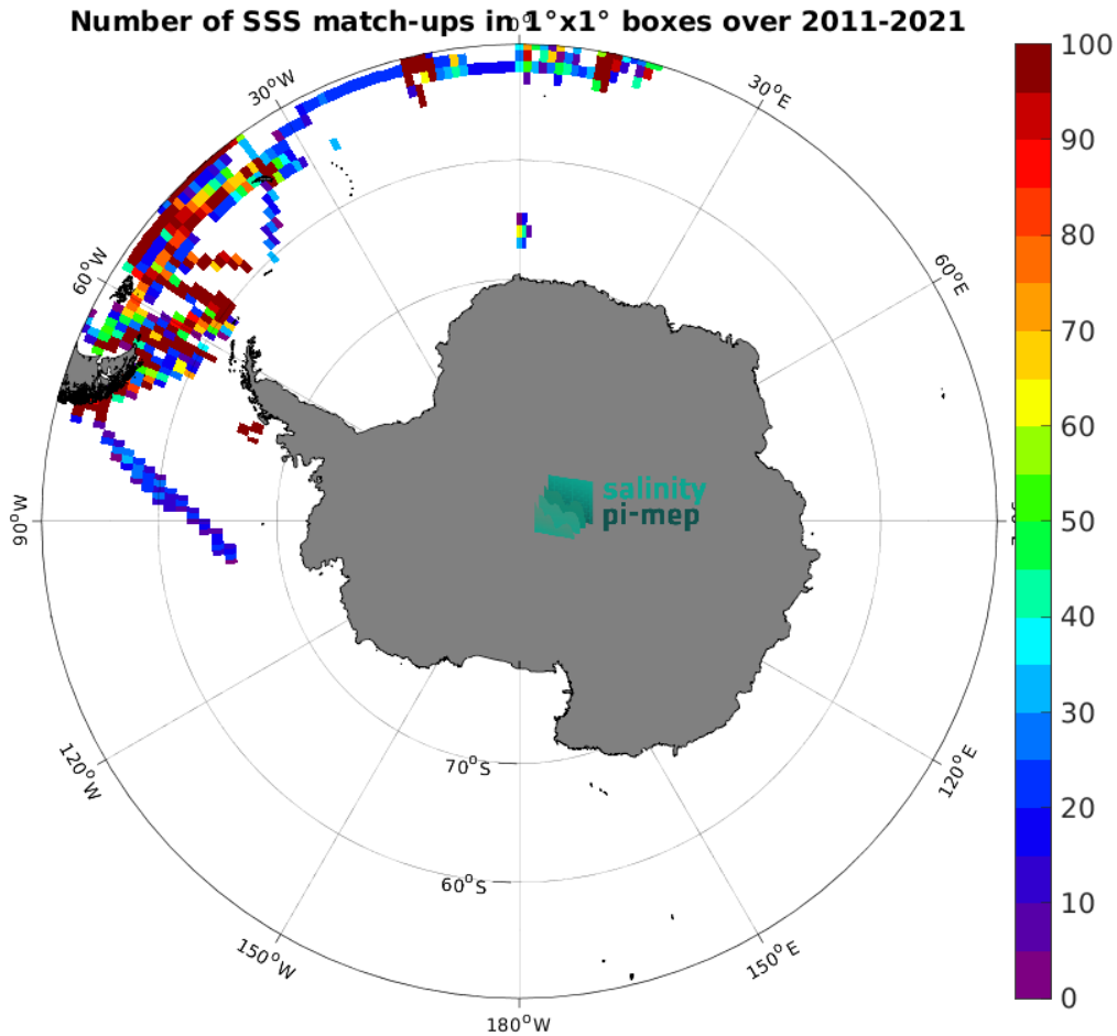
Figure 4: Number of SSS match-ups between TSG (Polarstern) SSS and the SMOS SSS L4 v2 - Daily (BEC) SSS product for the Southern Ocean Pi-MEP region over 1^\circ \times 1^\circ boxes and for the full satellite product period.
