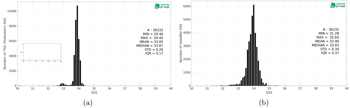
Figure 2: Histograms of SSS from TSG (Polarstern) (a) and SMOS SSS L4 v2 - Daily (BEC) (b) considering all match-up pairs per bins of 0.1 over the Southern Ocean Pi-MEP region and for the full satellite product period.
