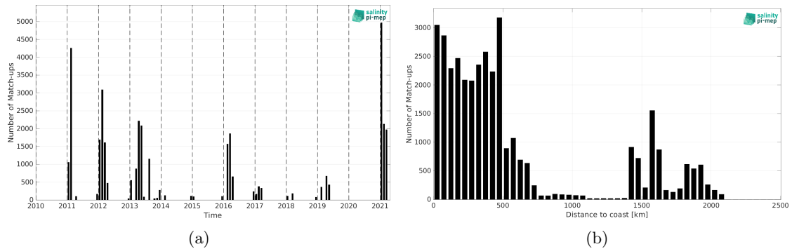
Figure 1: Number of match-ups between TSG (Polarstern) and SMOS SSS L4 v2 - Daily (BEC) SSS as a function of time (a) and as function of the distance to coast (b) over the Southern Ocean Pi-MEP region and for the full satellite product period.
