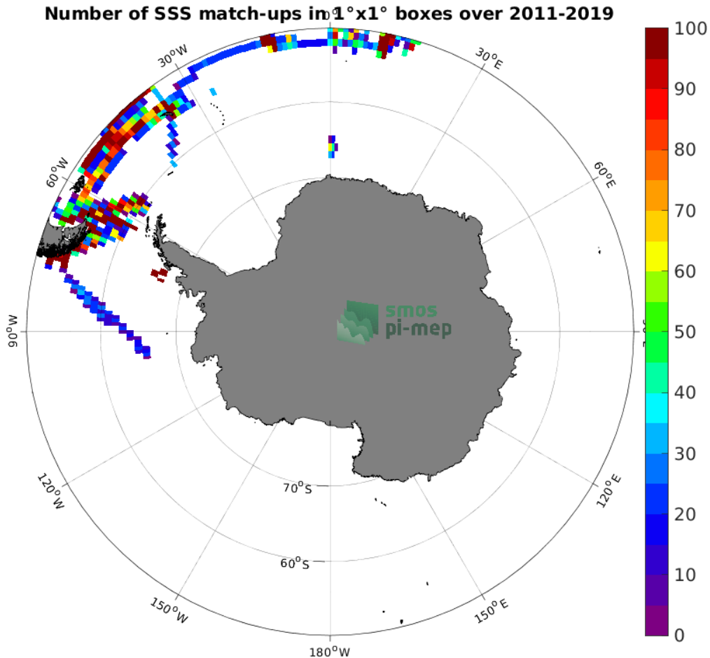
Figure 4: Number of SSS match-ups between TSG (Polarstern) SSS and the SMOS SSS L4 v2 - Daily (BEC) SSS product for the Southern Ocean Pi-MEP region over 1^\circ \times 1^\circ boxes and for the full satellite product period.
