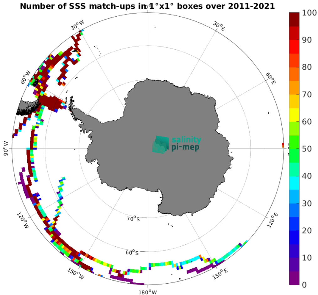
Figure 5: Number of SSS match-ups between TSG (GOSUD-Sailing-ship) SSS and the SMOS SSS L4 v2 - Daily (BEC) SSS product for the Southern Ocean Pi-MEP region over 1^\circ \times 1^\circ boxes and for the full satellite product period.
