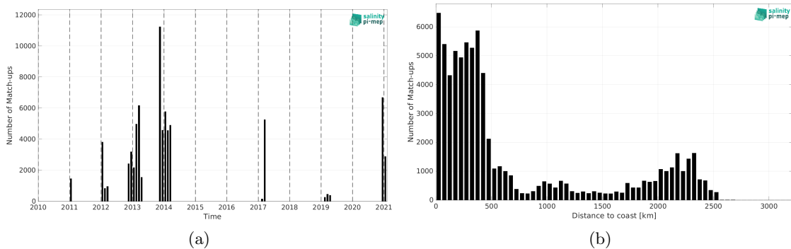
Figure 2: Number of match-ups between TSG (GOSUD-Sailing-ship) and SMOS SSS L4 v2 - Daily (BEC) SSS as a function of time (a) and as function of the distance to coast (b) over the Southern Ocean Pi-MEP region and for the full satellite product period.
