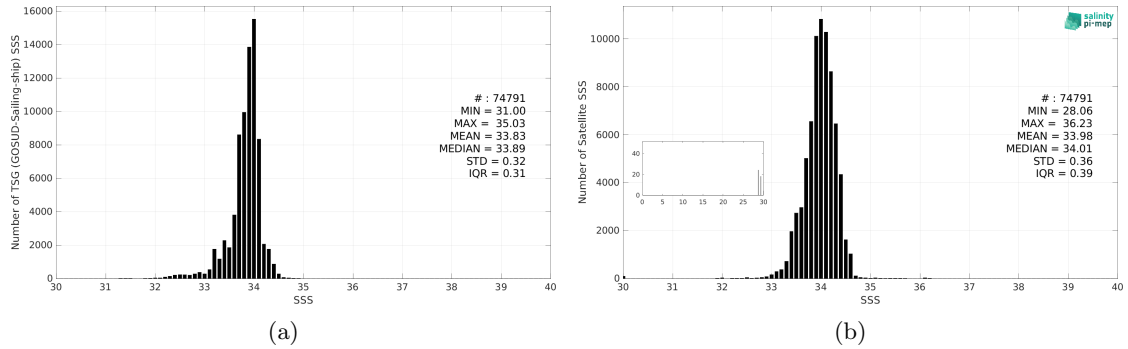
Figure 3: Histograms of SSS from TSG (GOSUD-Sailing-ship) (a) and SMOS SSS L4 v2 - Daily (BEC) (b) considering all match-up pairs per bins of 0.1 over the Southern Ocean Pi-MEP region and for the full satellite product period.
