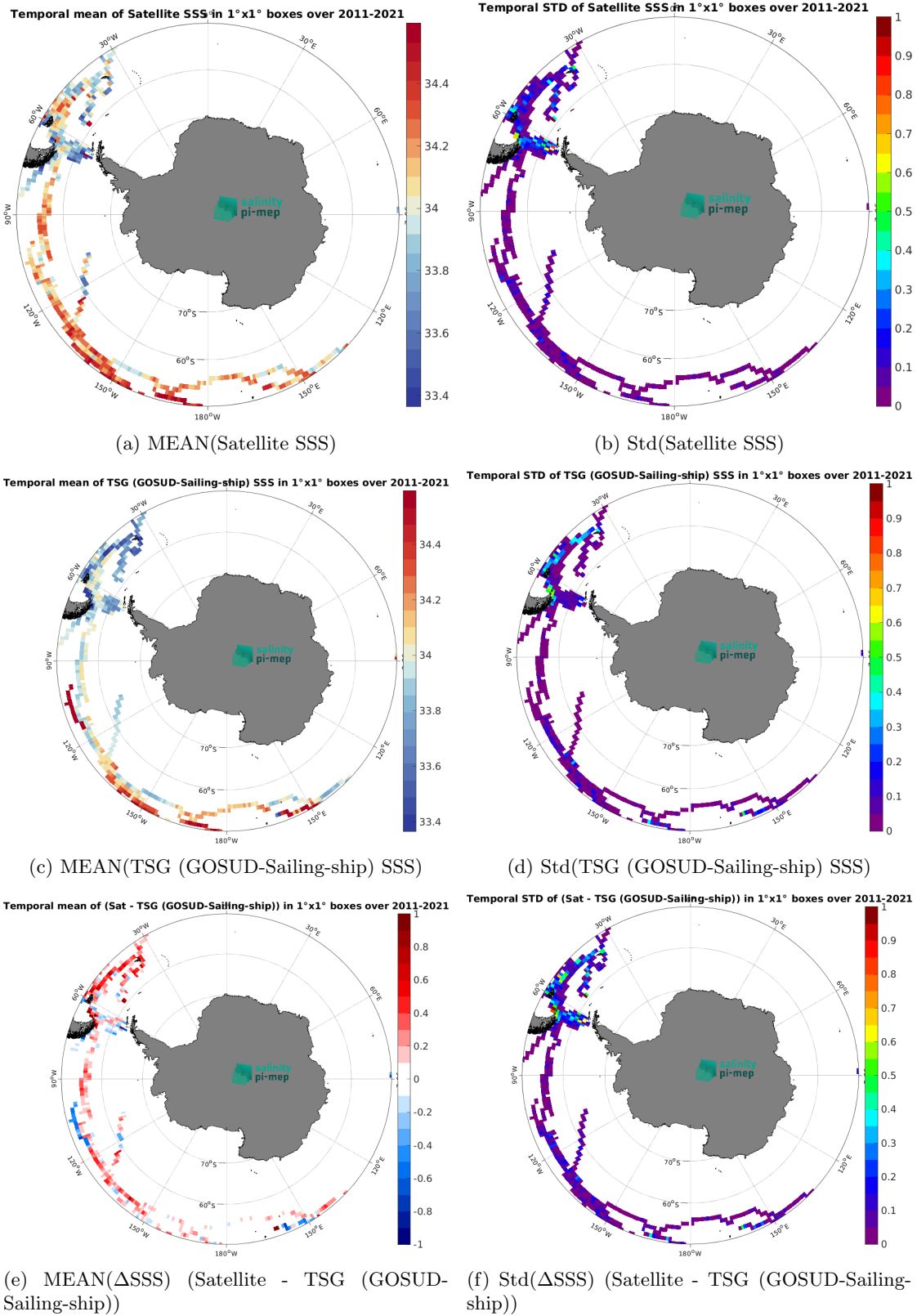
Figure 6: Temporal mean (left) and Std (right), of SSS from SMOS SSS L4 v2 - Daily (BEC) (top), TSG (GOSUD-Sailing-ship) (middle), and of \Delta SSS (Satellite - TSG (GOSUD-Sailing-ship)). Only match-up pairs are used to generate these maps.
