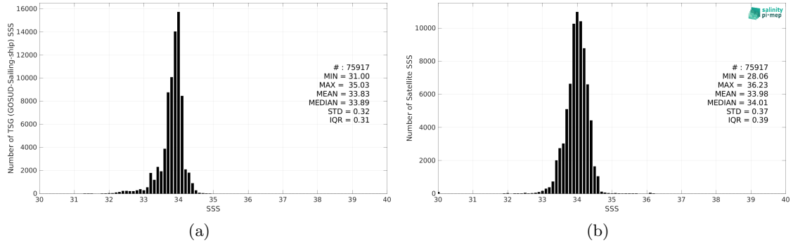
Figure 2: Histograms of SSS from TSG (GOSUD-Sailing-ship) (a) and SMOS SSS L4 v2 - Daily (BEC) (b) considering all match-up pairs per bins of 0.1 over the Southern Ocean Pi-MEP region and for the full satellite product period.
