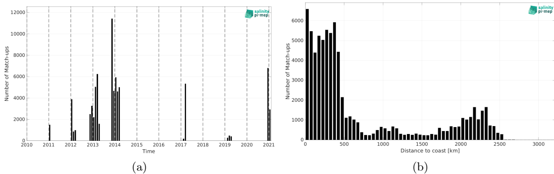
Figure 1: Number of match-ups between TSG (GOSUD-Sailing-ship) and SMOS SSS L4 v2 - Daily (BEC) SSS as a function of time (a) and as function of the distance to coast (b) over the Southern Ocean Pi-MEP region and for the full satellite product period.
