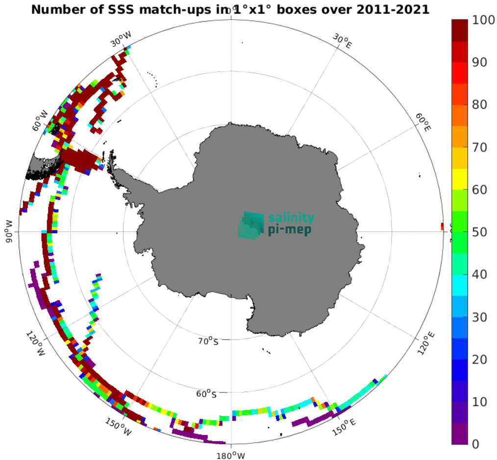
Figure 4: Number of SSS match-ups between TSG (GOSUD-Sailing-ship) SSS and the SMOS SSS L4 v2 - Daily (BEC) SSS product for the Southern Ocean Pi-MEP region over 1^\circ \times 1^\circ boxes and for the full satellite product period.
