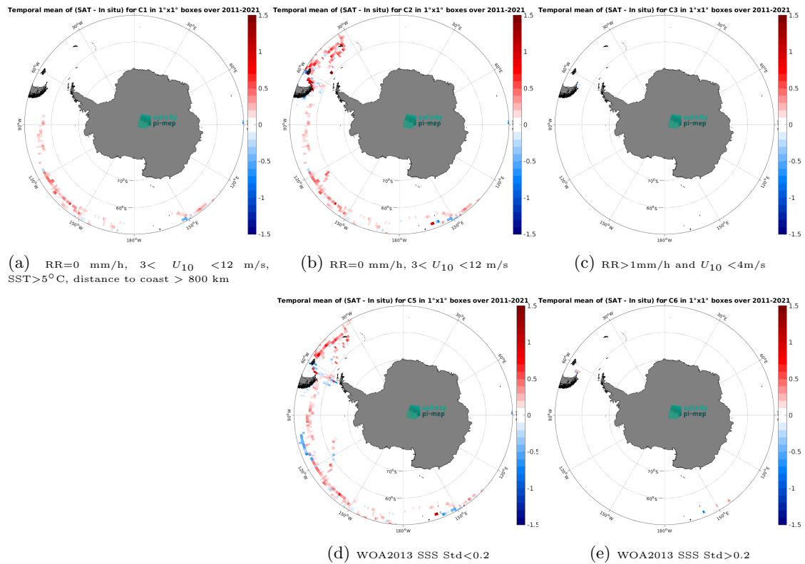
Figure 12: Temporal mean gridded over spatial boxes of size 1^\circ \times 1^\circ of \Delta\text{SSS} (SMOS SSS L4 v2 - Daily (BEC) - TSG (GOSUD-Sailing-ship)) for 5 different subdatasets corresponding to: RR=0 mm/h, 3 < U_{10} < 12 m/s, SST > 5^\circ\text{C} , distance to coast > 800 km (a), RR=0 mm/h, 3 < U_{10} < 12 m/s (b), RR > 1 mm/h and U_{10} < 4 m/s (c), WOA2013 SSS Std < 0.2 (d), WOA2013 SSS Std > 0.2 (e).
