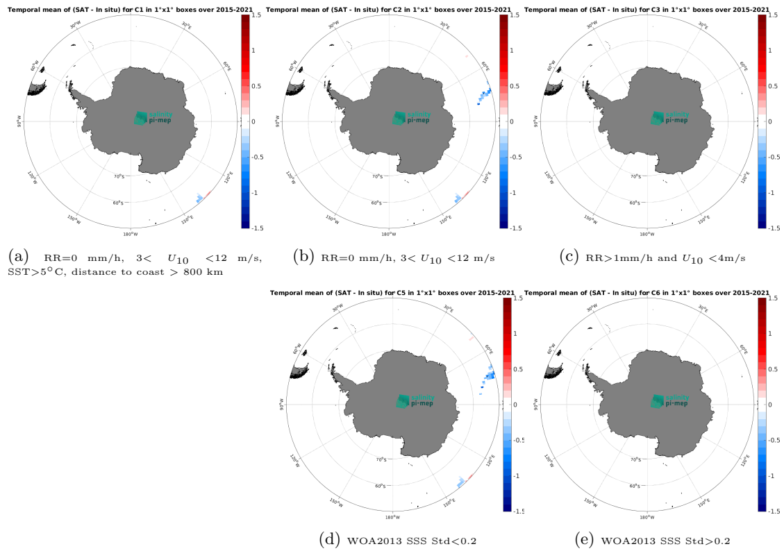
Figure 12: Temporal mean gridded over spatial boxes of size 1^\circ \times 1^\circ of \Delta\text{SSS} (SMOS SSS L4 v2 - Daily (BEC) - TSG (GOSUD-Research-vessel)) for 5 different subdatasets corresponding to: RR=0 mm/h, 3 < U_{10} < 12 m/s, SST > 5^\circ\text{C} , distance to coast > 800 km (a), RR=0 mm/h, 3 < U_{10} < 12 m/s (b), RR > 1 mm/h and U_{10} < 4 m/s (c), WOA2013 SSS Std < 0.2 (d), WOA2013 SSS Std > 0.2 (e).
