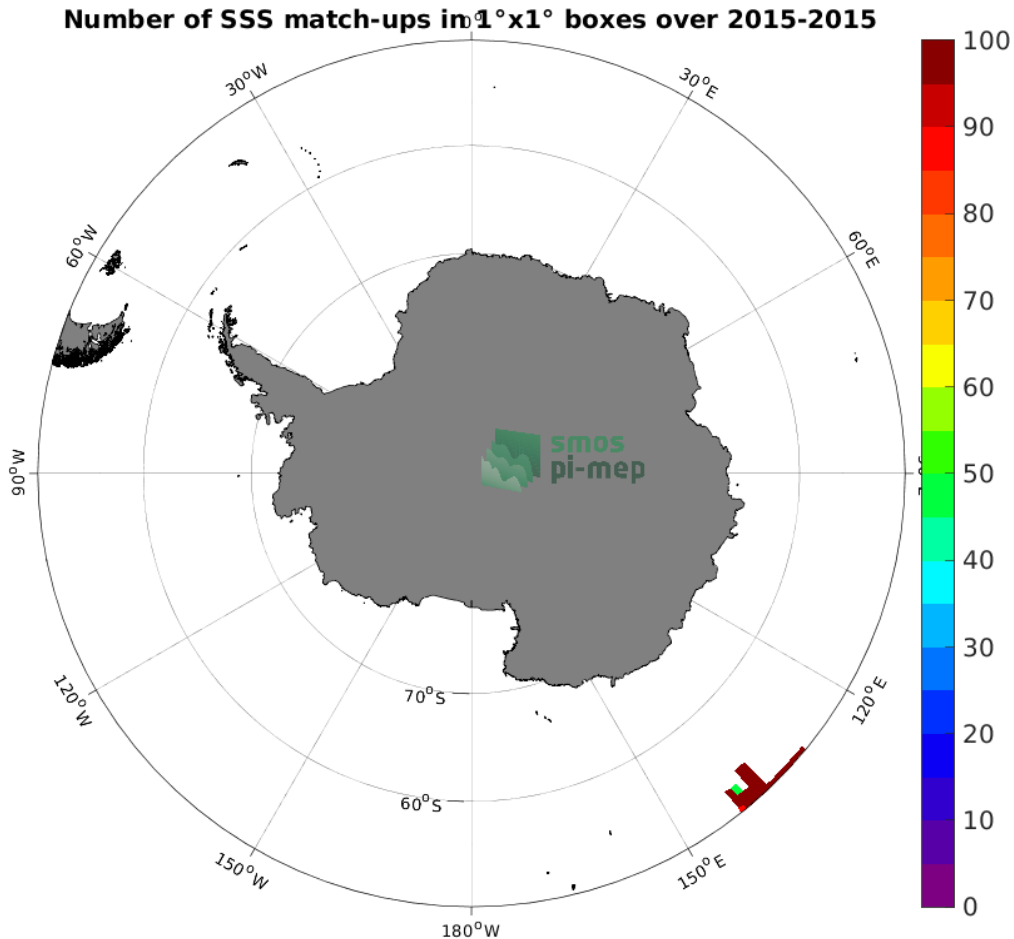
Figure 4: Number of SSS match-ups between TSG (GOSUD-Research-vessel) SSS and the SMOS SSS L4 v2 - Daily (BEC) SSS product for the Southern Ocean Pi-MEP region over 1^\circ \times 1^\circ boxes and for the full satellite product period.
