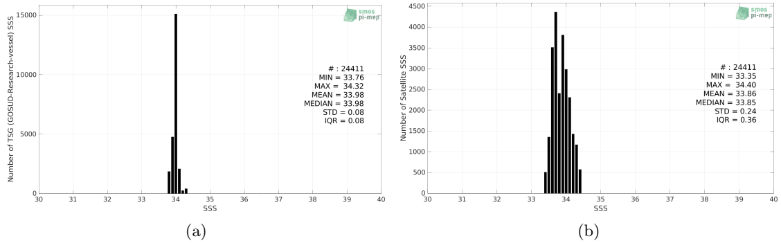
Figure 2: Histograms of SSS from TSG (GOSUD-Research-vessel) (a) and SMOS SSS L4 v2 - Daily (BEC) (b) considering all match-up pairs per bins of 0.1 over the Southern Ocean Pi-MEP region and for the full satellite product period.
