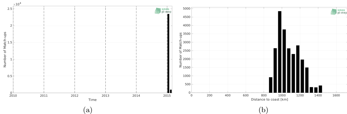
Figure 1: Number of match-ups between TSG (GOSUD-Research-vessel) and SMOS SSS L4 v2 - Daily (BEC) SSS as a function of time (a) and as function of the distance to coast (b) over the Southern Ocean Pi-MEP region and for the full satellite product period.
