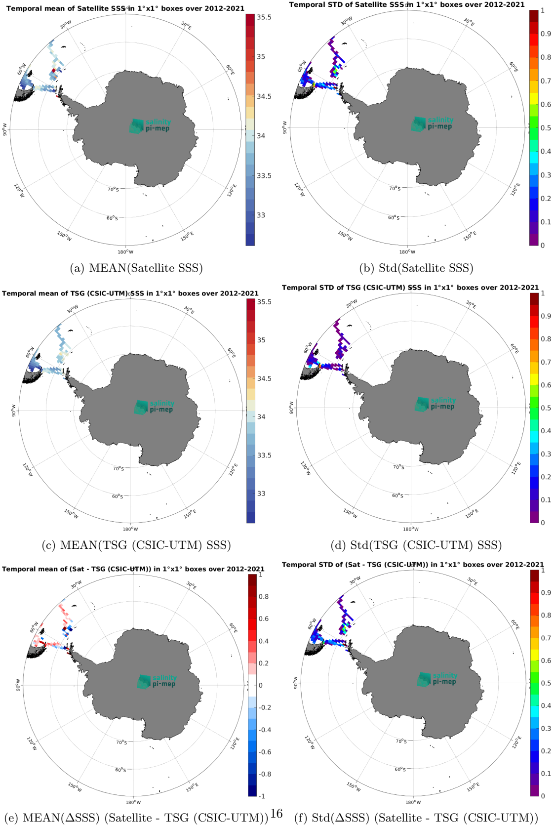
Figure 7: Temporal mean (left) and Std (right) of SSS from SMOS SSS L4 v2 - Daily (BEC) (top), TSG (CSIC-UTM) (middle), and of \Delta SSS (Satellite - TSG (CSIC-UTM)). Only match-up pairs are used to generate these maps.
