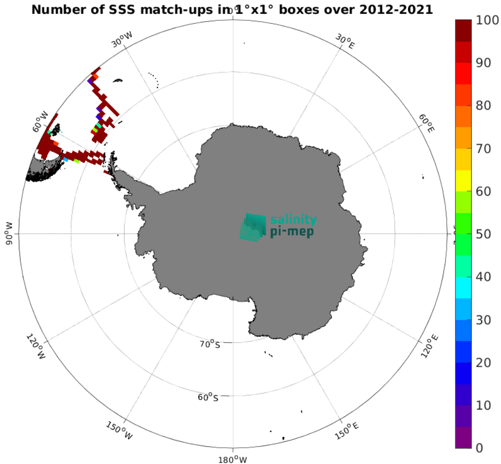
Figure 5: Number of SSS match-ups between TSG (CSIC-UTM) SSS and the SMOS SSS L4 v2 - Daily (BEC) SSS product for the Southern Ocean Pi-MEP region over 1^\circ \times 1^\circ boxes and for the full satellite product period.
