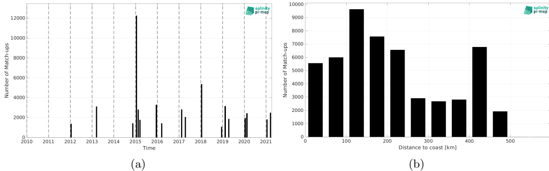
Figure 2: Number of match-ups between TSG (CSIC-UTM) and SMOS SSS L4 v2 - Daily (BEC) SSS as a function of time (a) and as function of the distance to coast (b) over the Southern Ocean Pi-MEP region and for the full satellite product period.
