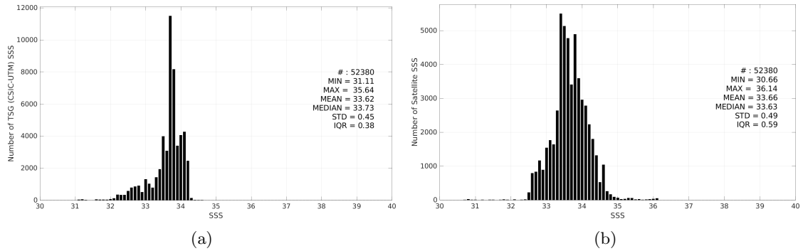
Figure 3: Histograms of SSS from TSG (CSIC-UTM) (a) and SMOS SSS L4 v2 - Daily (BEC) (b) considering all match-up pairs per bins of 0.1 over the Southern Ocean Pi-MEP region and for the full satellite product period.
