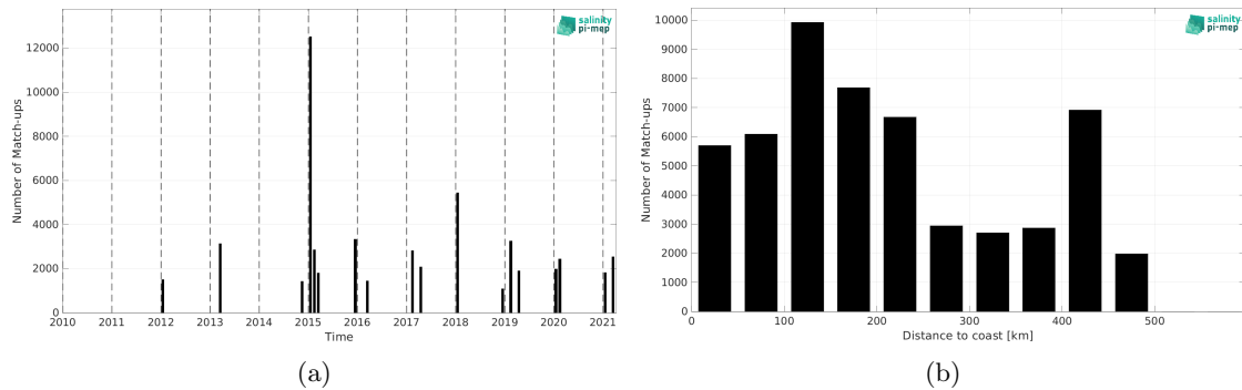
Figure 1: Number of match-ups between TSG (CSIC-UTM) and SMOS SSS L4 v2 - Daily (BEC) SSS as a function of time (a) and as function of the distance to coast (b) over the Southern Ocean Pi-MEP region and for the full satellite product period.
