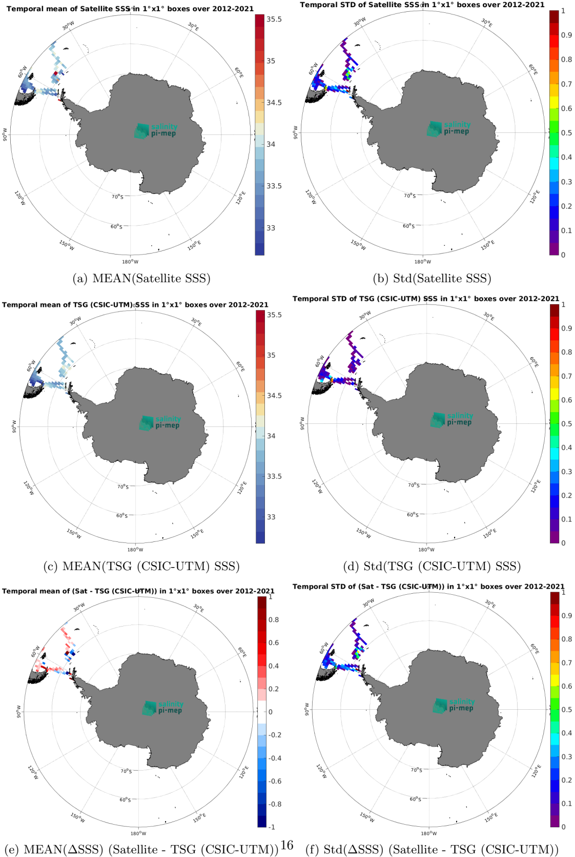
Figure 6: Temporal mean (left) and Std (right) of SSS from SMOS SSS L4 v2 - Daily (BEC) (top), TSG (CSIC-UTM) (middle), and of \Delta SSS (Satellite - TSG (CSIC-UTM)). Only match-up pairs are used to generate these maps.
