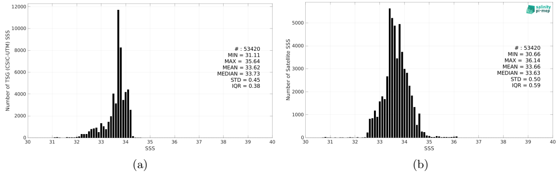
Figure 2: Histograms of SSS from TSG (CSIC-UTM) (a) and SMOS SSS L4 v2 - Daily (BEC) (b) considering all match-up pairs per bins of 0.1 over the Southern Ocean Pi-MEP region and for the full satellite product period.
