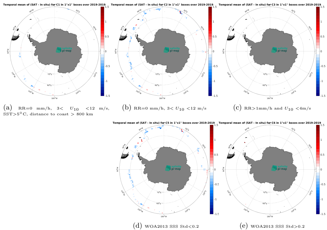
Figure 14: Temporal mean gridded over spatial boxes of size 1^\circ \times 1^\circ of \Delta SSS (SMOS SSS L4 v2 - Daily (BEC) - Saikrone) for 5 different subdatasets corresponding to: RR=0 mm/h, 3 < U_{10} < 12 m/s, SST > 5^\circ\text{C} , distance to coast > 800 km (a), RR=0 mm/h, 3 < U_{10} < 12 m/s (b), RR > 1 mm/h and U_{10} < 4 m/s (c), WOA2013 SSS Std < 0.2 (d), WOA2013 SSS Std > 0.2 (e).
