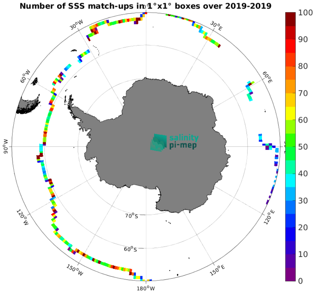
Figure 5: Number of SSS match-ups between Saildrone SSS and the SMOS SSS L4 v2 - Daily (BEC) SSS product for the Southern Ocean Pi-MEP region over 1^\circ \times 1^\circ boxes and for the full satellite product period.
