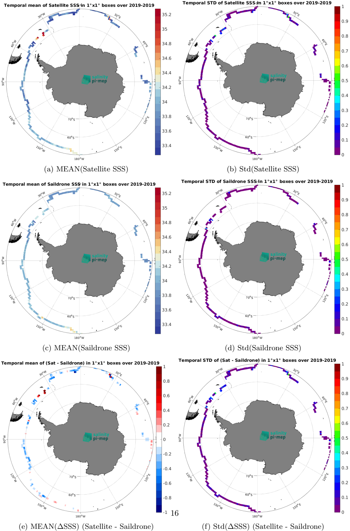
Figure 7: Temporal mean (left) and Std (right) of SSS from SMOS SSS L4 v2 - Daily (BEC) (top), Saildrone (middle), and of \Delta SSS (Satellite - Saildrone). Only match-up pairs are used to generate these maps.
