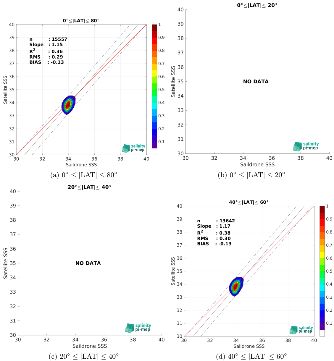
Figure 10: Contour maps of the concentration of SMOS SSS L4 v2 - Daily (BEC) SSS (y-axis) versus Saldrone SSS (x-axis) at match-up pairs for different latitude bands. For each plot, the red line shows x=y . The black thin and dashed lines indicate a linear fit through the data cloud and the \pm 95\% confidence levels, respectively. The number match-up pairs n , the slope and R^2 coefficient of the linear fit, the root mean square (RMS) and the mean bias between satellite and in situ data are indicated for each latitude band in each plots.
