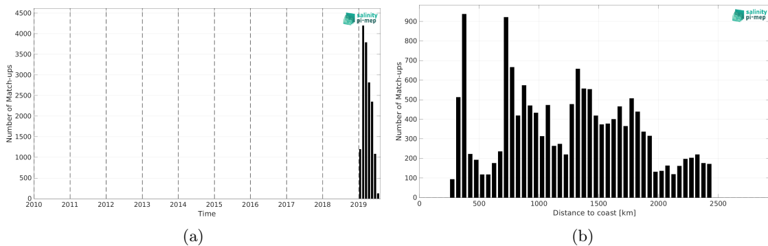
Figure 2: Number of match-ups between Saildrone and SMOS SSS L4 v2 - Daily (BEC) SSS as a function of time (a) and as function of the distance to coast (b) over the Southern Ocean Pi-MEP region and for the full satellite product period.
