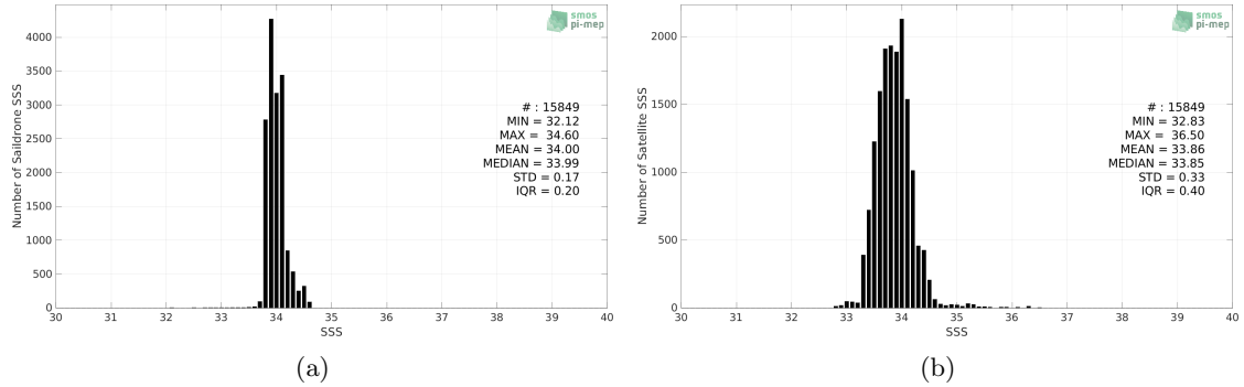
Figure 2: Histograms of SSS from Sairdrone (a) and SMOS SSS L4 v2 - Daily (BEC) (b) considering all match-up pairs per bins of 0.1 over the Southern Ocean Pi-MEP region and for the full satellite product period.
