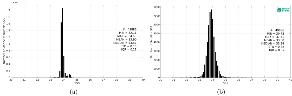
Figure 2: Histograms of SSS from Marine mammals (a) and SMOS SSS L4 v2 - Daily (BEC) (b) considering all match-up pairs per bins of 0.1 over the Southern Ocean Pi-MEP region and for the full satellite product period.
