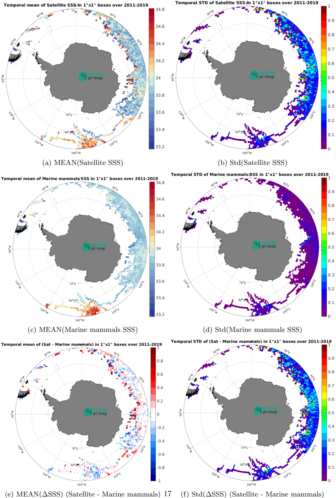
Figure 6: Temporal mean (left) and Std (right) of SSS from SMOS SSS L4 v2 - Daily (BEC) (top), Marine mammals (middle), and of \Delta SSS (Satellite - Marine mammals). Only match-up pairs are used to generate these maps.
