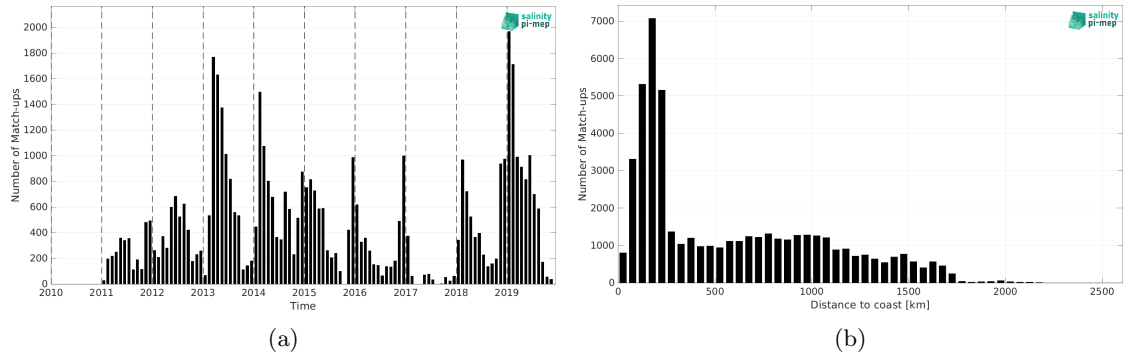
Figure 1: Number of match-ups between Marine mammals and SMOS SSS L4 v2 - Daily (BEC) SSS as a function of time (a) and as function of the distance to coast (b) over the Southern Ocean Pi-MEP region and for the full satellite product period.
