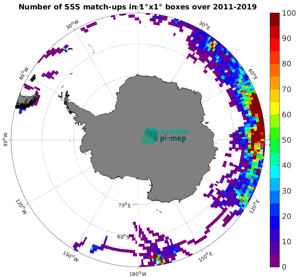
Figure 4: Number of SSS match-ups between Marine mammals SSS and the SMOS SSS L4 v2 - Daily (BEC) SSS product for the Southern Ocean Pi-MEP region over 1^\circ \times 1^\circ boxes and for the full satellite product period.
