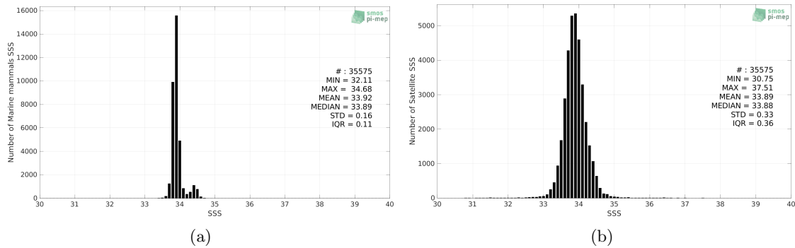
Figure 2: Histograms of SSS from Marine mammals (a) and SMOS SSS L4 v2 - Daily (BEC) (b) considering all match-up pairs per bins of 0.1 over the Southern Ocean Pi-MEP region and for the full satellite product period.
