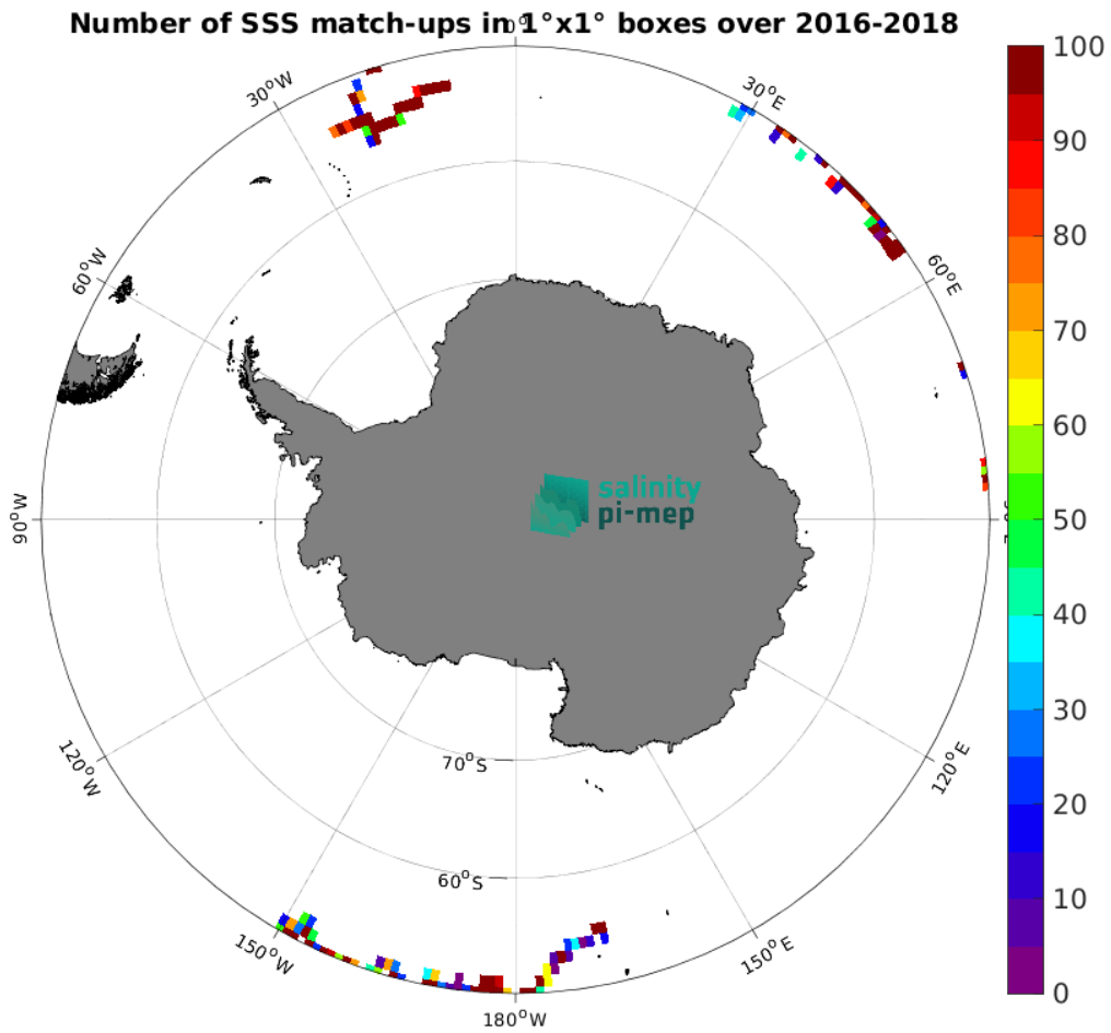
Figure 4: Number of SSS match-ups between Surface drifters SSS and the SMOS SSS L4 v2 - Daily (BEC) SSS product for the Southern Ocean Pi-MEP region over 1^\circ \times 1^\circ boxes and for the full satellite product period.
