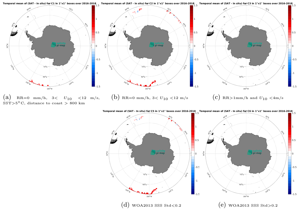
Figure 13: Temporal mean gridded over spatial boxes of size 1^\circ \times 1^\circ of \Delta SSS (SMOS SSS L4 v2 - Daily (BEC) - Surface drifters) for 5 different subdatasets corresponding to:RR=0 mm/h, 3 < U_{10} < 12 m/s, SST > 5^\circ\text{C} , distance to coast > 800 km (a), RR=0 mm/h, 3 < U_{10} < 12 m/s (b), RR > 1 mm/h and U_{10} < 4 m/s (c), WOA2013 SSS Std < 0.2 (d), WOA2013 SSS Std > 0.2 (e).
