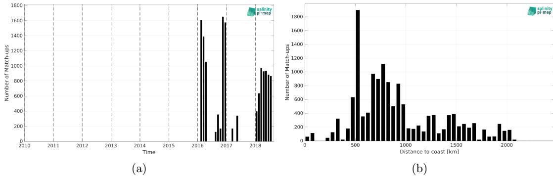
Figure 2: Number of match-ups between Surface drifters and SMOS SSS L4 v2 - Daily (BEC) SSS as a function of time (a) and as function of the distance to coast (b) over the Southern Ocean Pi-MEP region and for the full satellite product period.
