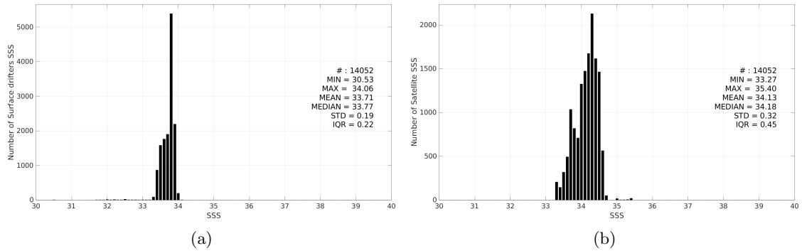
Figure 3: Histograms of SSS from Surface drifters (a) and SMOS SSS L4 v2 - Daily (BEC) (b) considering all match-up pairs per bins of 0.1 over the Southern Ocean Pi-MEP region and for the full satellite product period.
