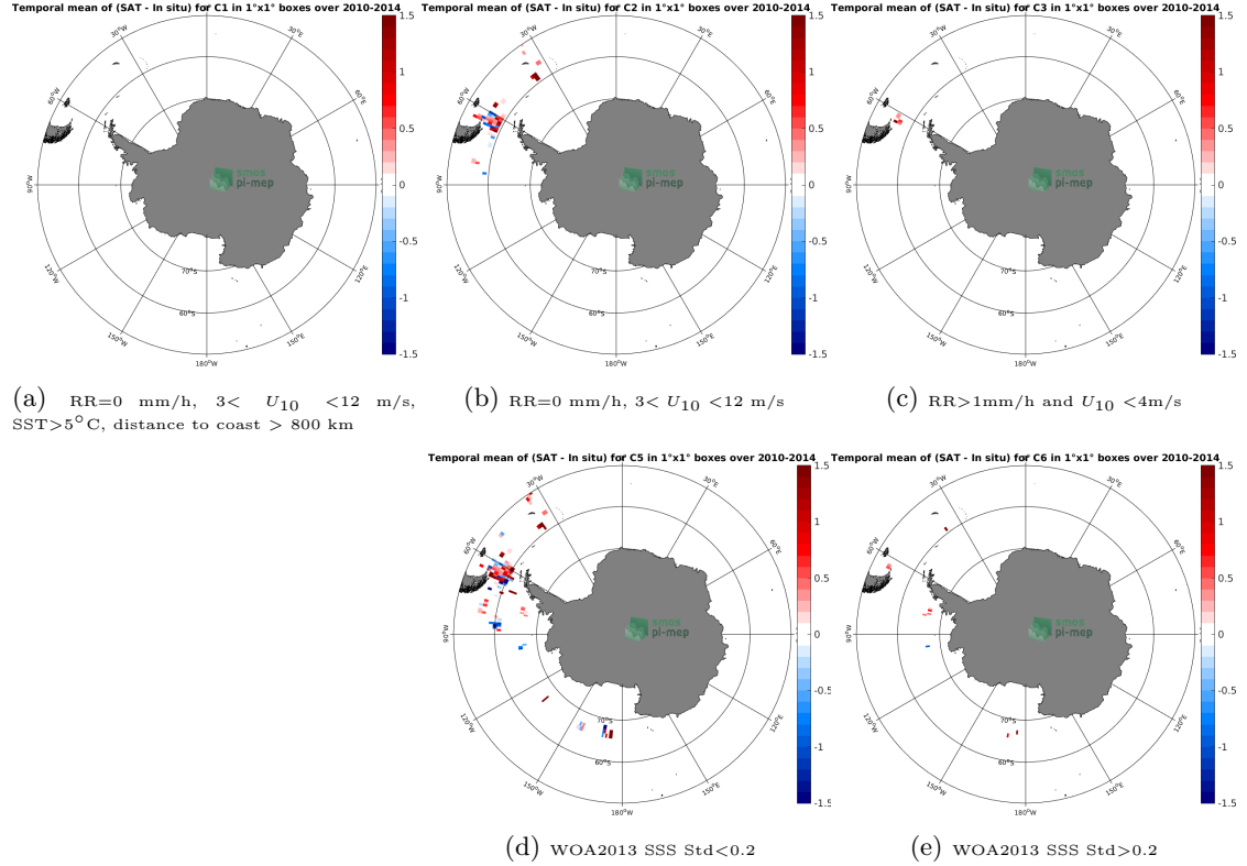
Figure 12: Temporal mean gridded over spatial boxes of size 1^{\circ} \times 1^{\circ} of \Delta\text{SSS} (SMOS SSS L3 v3 Monthly (ICDC) - TSG (SAMOS)) for 5 different subdatasets corresponding to: RR=0 mm/h, 3 < U_{10} < 12 m/s, SST > 5^{\circ}\text{C} , distance to coast > 800 km (a), RR=0 mm/h, 3 < U_{10} < 12 m/s (b), RR > 1 mm/h and U_{10} < 4 m/s (c), WOA2013 SSS Std < 0.2 (d), WOA2013 SSS Std > 0.2 (e).
