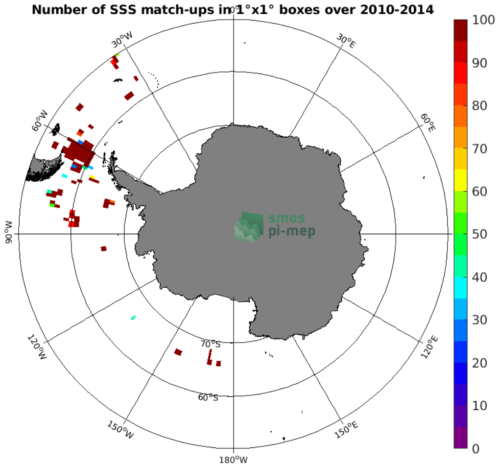
Figure 4: Number of SSS match-ups between TSG (SAMOS) SSS and the SMOS SSS L3 v3 Monthly (ICDC) SSS product for the Southern Ocean Pi-MEP region over 1^\circ \times 1^\circ boxes and for the full satellite product period.
