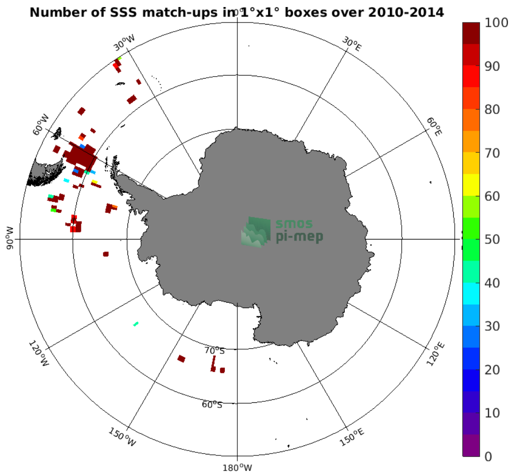
Figure 4: Number of SSS match-ups between TSG (SAMOS) SSS and the SMOS SSS L3 v3 Monthly (ICDC) SSS product for the Southern Ocean Pi-MEP region over 1^\circ \times 1^\circ boxes and for the full satellite product period.
