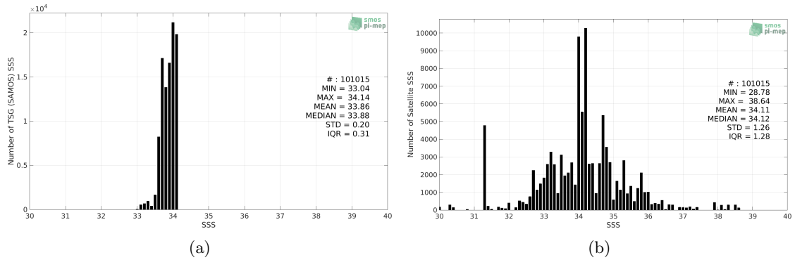
Figure 2: Histograms of SSS from TSG (SAMOS) (a) and SMOS SSS L3 v3 Monthly (ICDC) (b) considering all match-up pairs per bins of 0.1 over the Southern Ocean Pi-MEP region and for the full satellite product period.
