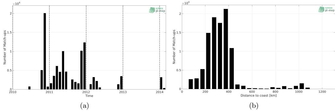
Figure 1: Number of match-ups between TSG (SAMOS) and SMOS SSS L3 v3 Monthly (ICDC) SSS as a function of time (a) and as function of the distance to coast (b) over the Southern Ocean Pi-MEP region and for the full satellite product period.
