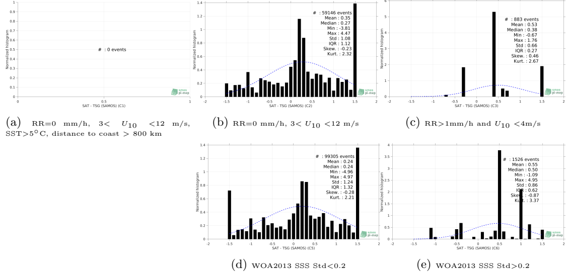
Figure 13: Normalized histogram of \Delta\text{SSS} (SMOS SSS L3 v3 Monthly (ICDC) - TSG (SAMOS)) for 5 different subdatasets corresponding to: RR=0 mm/h, 3 < U_{10} < 12 m/s, SST > 5^\circ\text{C} , distance to coast > 800 km (a), RR=0 mm/h, 3 < U_{10} < 12 m/s (b), RR > 1\text{mm/h} and U_{10} < 4\text{m/s} (c), WOA2013 SSS Std < 0.2 (d), WOA2013 SSS Std > 0.2 (e).
