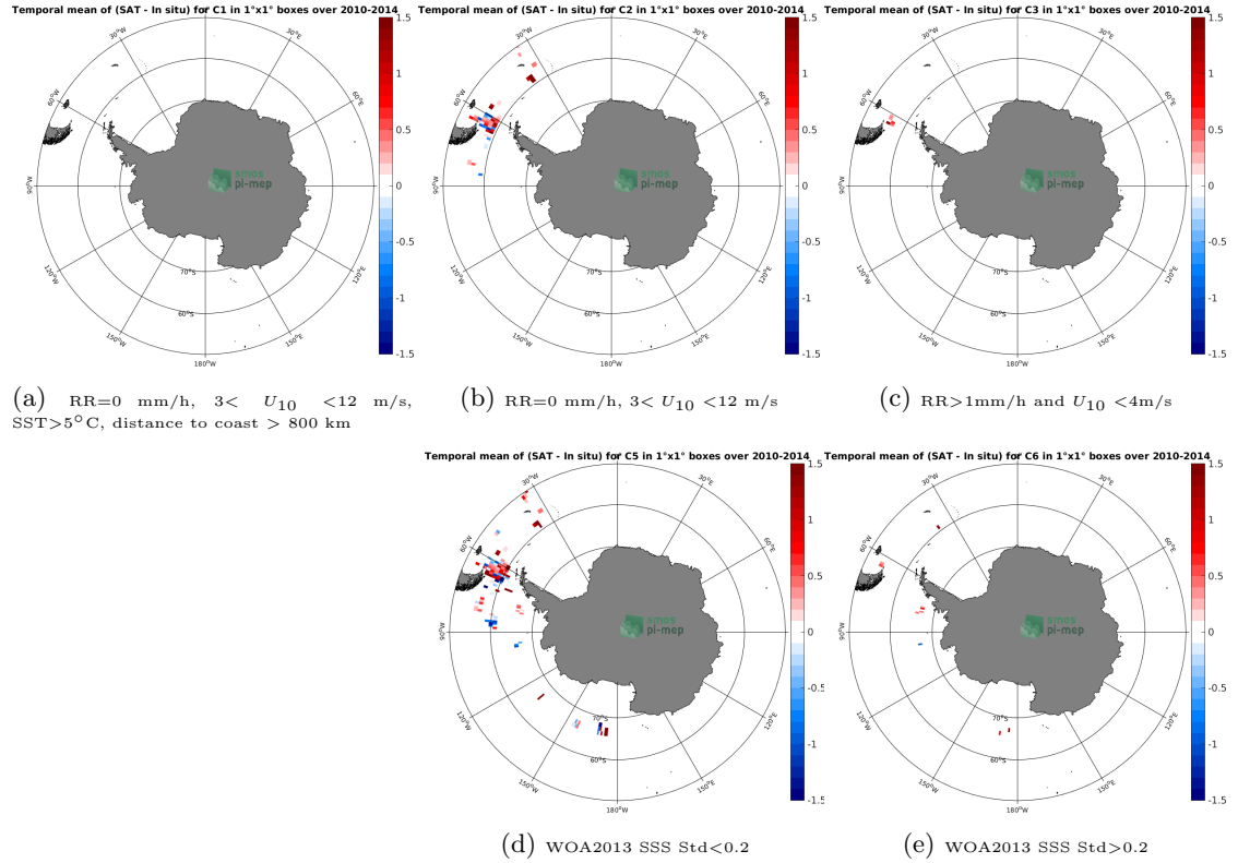
Figure 12: Temporal mean gridded over spatial boxes of size 1^{\circ}\times 1^{\circ} of \Delta\text{SSS} (SMOS-L3-ICDC-V3-MONTHLY-0.5DEG - TSG-SAMOS) for 5 different subdatasets corresponding to:RR=0 mm/h, 3 < U_{10} < 12 m/s, SST >5^{\circ}\text{C} , distance to coast > 800 km (a), RR=0 mm/h, 3 < U_{10} < 12 m/s (b), RR >1 mm/h and U_{10} < 4 m/s (c), WOA2013 SSS Std <0.2 (d), WOA2013 SSS Std >0.2 (e).
