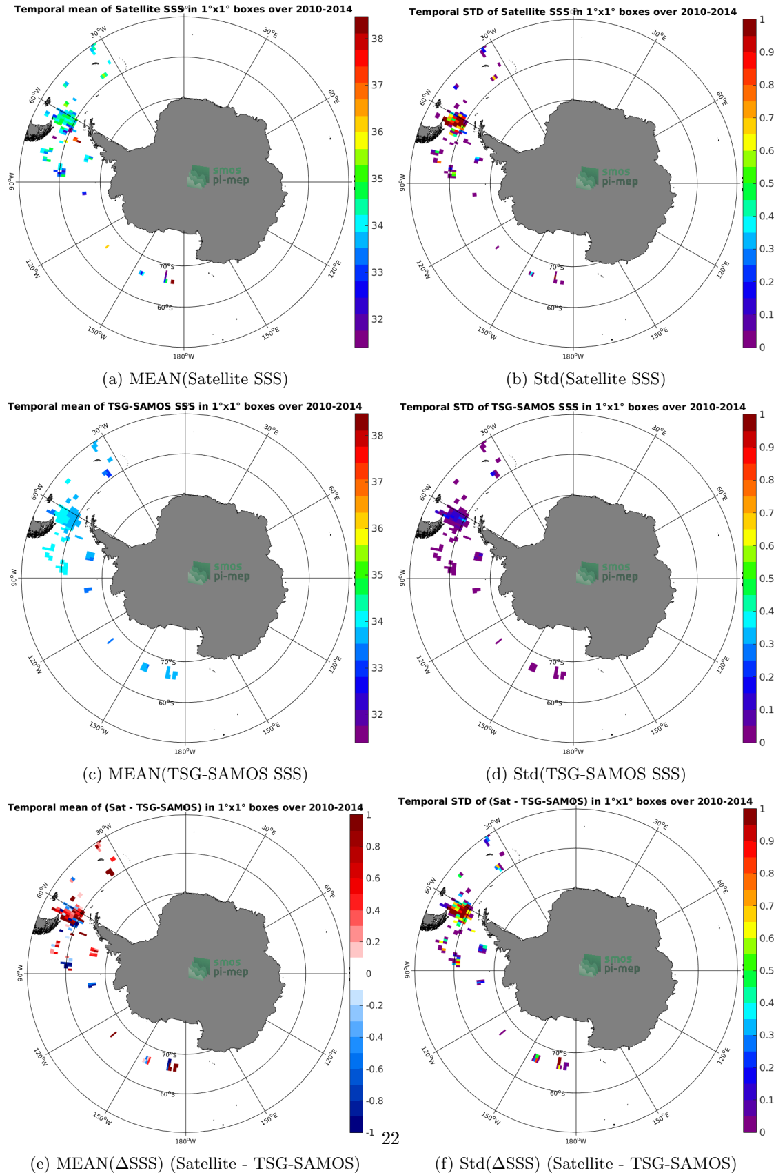
Figure 6: Temporal mean (left) and Std (right) of SSS from SMOS-L3-ICDC-V3-MONTHLY-0.5DEG (top), TSG-SAMOS (middle), and of \Delta SSS (Satellite - TSG-SAMOS). Only match-up pairs are used to generate these maps.
