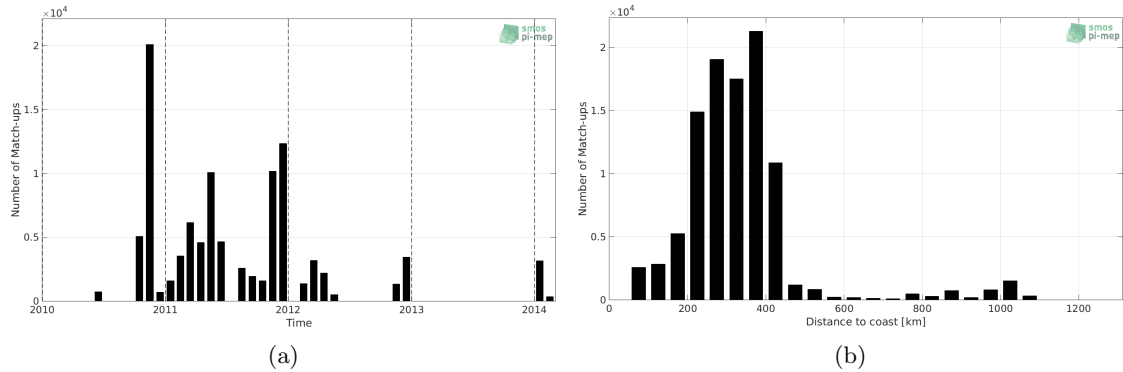
Figure 1: Number of match-ups between TSG-SAMOS and SMOS-L3-ICDC-V3-MONTHLY-0.5DEG SSS as a function of time (a) and as function of the distance to coast (b) over the Southern Ocean Pi-MEP region and for the full satellite product period.
