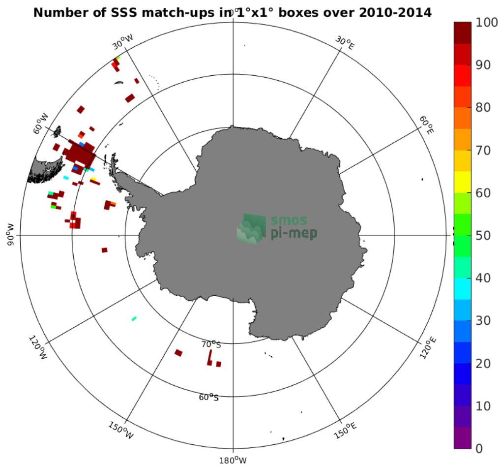
Figure 4: Number of SSS match-ups between TSG-SAMOS SSS and the SMOS-L3-ICDC-V3-MONTHLY-0.5DEG SSS product for the Southern Ocean Pi-MEP region over 1^\circ \times 1^\circ boxes and for the full satellite product period.
