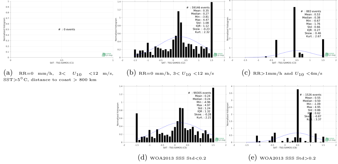
Figure 13: Normalized histogram of \Delta\text{SSS} (SMOS-L3-ICDC-V3-MONTHLY-0.5DEG - TSG-SAMOS) for 5 different subdatasets corresponding to: RR=0 mm/h, 3 < U_{10} < 12 m/s, SST > 5^\circ\text{C} , distance to coast > 800 km (a), RR=0 mm/h, 3 < U_{10} < 12 m/s (b), RR > 1\text{mm/h} and U_{10} < 4\text{m/s} (c), WOA2013 SSS Std<0.2 (d), WOA2013 SSS Std>0.2 (e).
