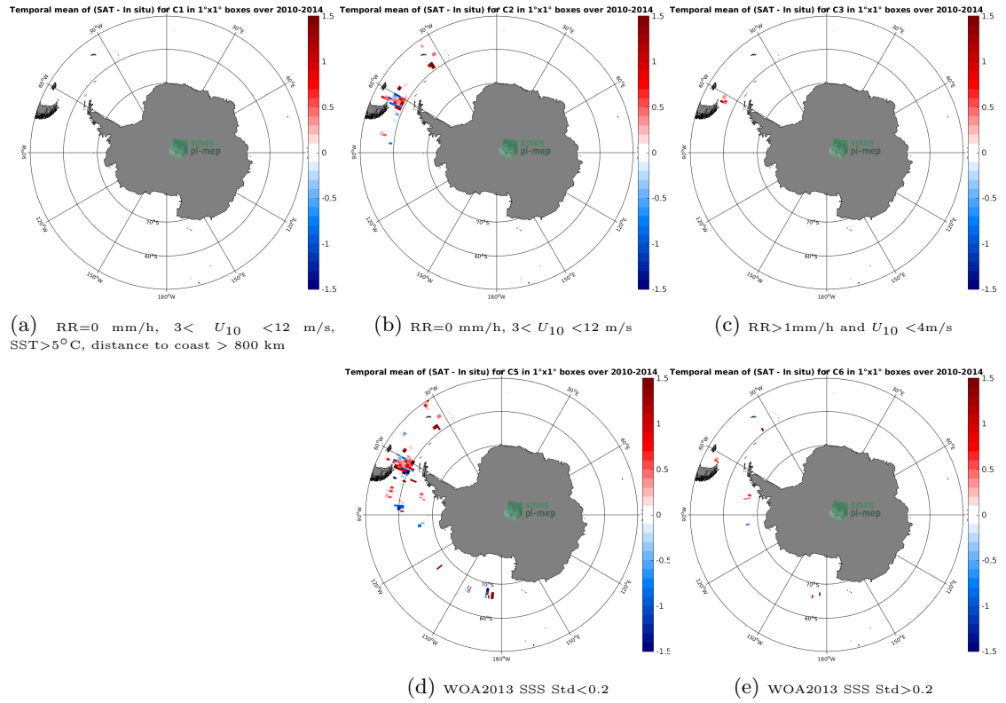
Figure 12: Temporal mean gridded over spatial boxes of size 1^\circ \times 1^\circ of \Delta SSS (SMOS-L3-ICDC-V3-MONTHLY-0.5DEG - TSG-SAMOS) for 5 different subdatasets corresponding to: RR=0 mm/h, 3 < U_{10} < 12 m/s, SST > 5^\circ\text{C} , distance to coast > 800 km (a), RR=0 mm/h, 3 < U_{10} < 12 m/s (b), RR > 1 mm/h and U_{10} < 4 m/s (c), WOA2013 SSS Std < 0.2 (d), WOA2013 SSS Std > 0.2 (e).
