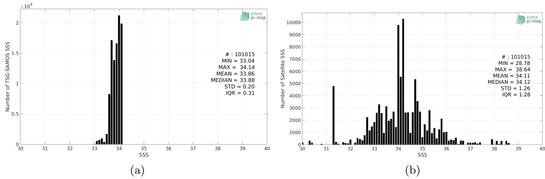
Figure 2: Histograms of SSS from TSG-SAMOS (a) and SMOS-L3-ICDC-V3-MONTHLY-0.5DEG (b) considering all match-up pairs per bins of 0.1 over the Southern Ocean Pi-MEP region and for the full satellite product period.
