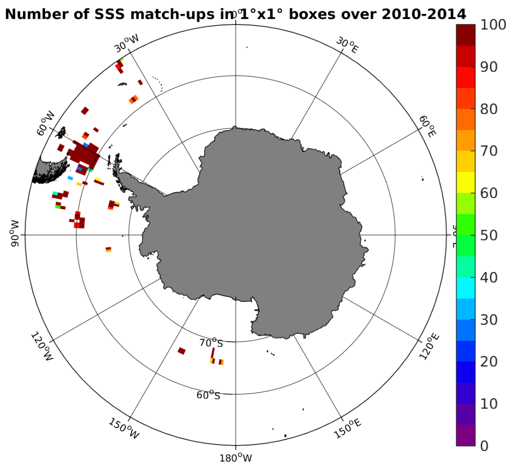
Figure 4: Number of SSS match-ups between TSG-SAMOS SSS and the SMOS-L3-ICDC-V3-MONTHLY-0.5DEG SSS product for the Southern Ocean Pi-MEP region over 1^\circ \times 1^\circ boxes and for the full satellite product period.
