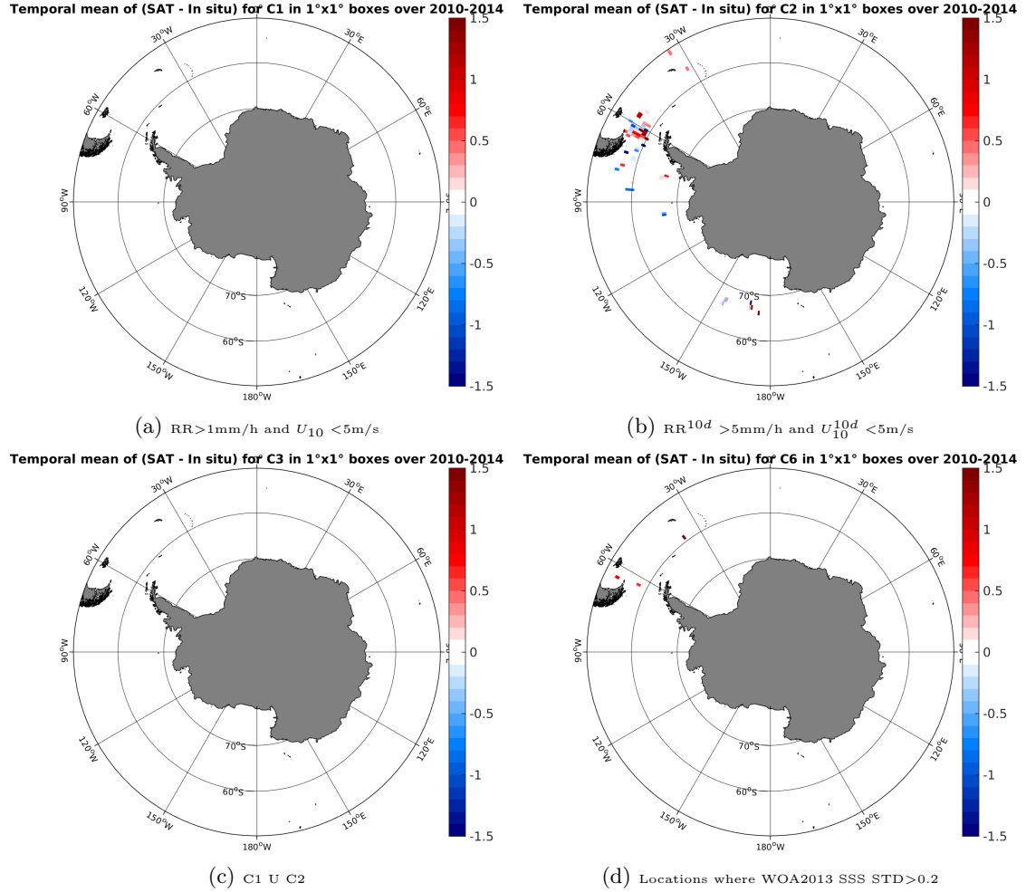
Figure 12: Temporal mean gridded over spatial boxes of size 1^\circ \times 1^\circ of \Delta SSS (SMOS-L3-ICDC-V3-MONTHLY-0.5DEG - TSG-SAMOS) for 4 different subdatasets corresponding to: RR > 1mm/h and U_{10} < 5\text{m/s} (a), RR 10d > 5mm/h and U_{10}^{10d} < 5\text{m/s} (b), C1 U C2 (c), Locations where WOA2013 SSS STD > 0.2 (d).
