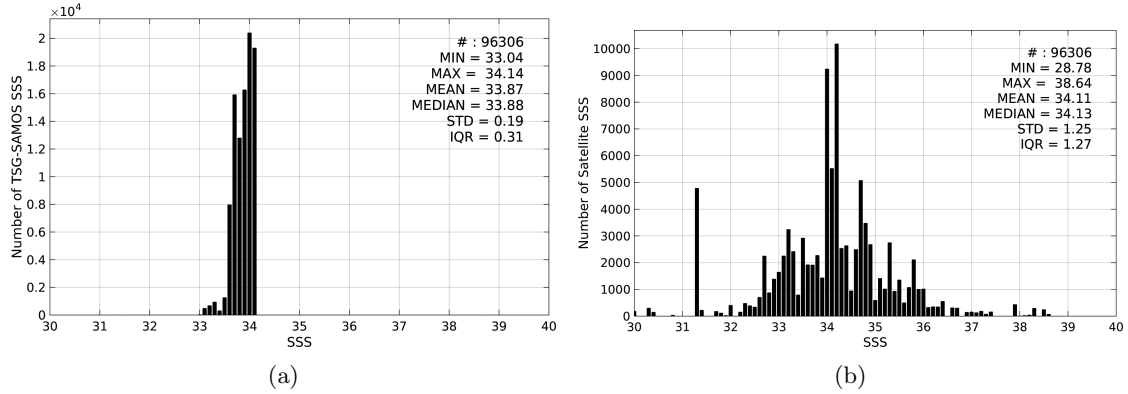
Figure 2: Histograms of SSS from TSG-SAMOS (a) and SMOS-L3-ICDC-V3-MONTHLY-0.5DEG (b) considering all match-up pairs per bins of 0.1 over the Southern Ocean Pi-MEP region and for the full satellite product period.
