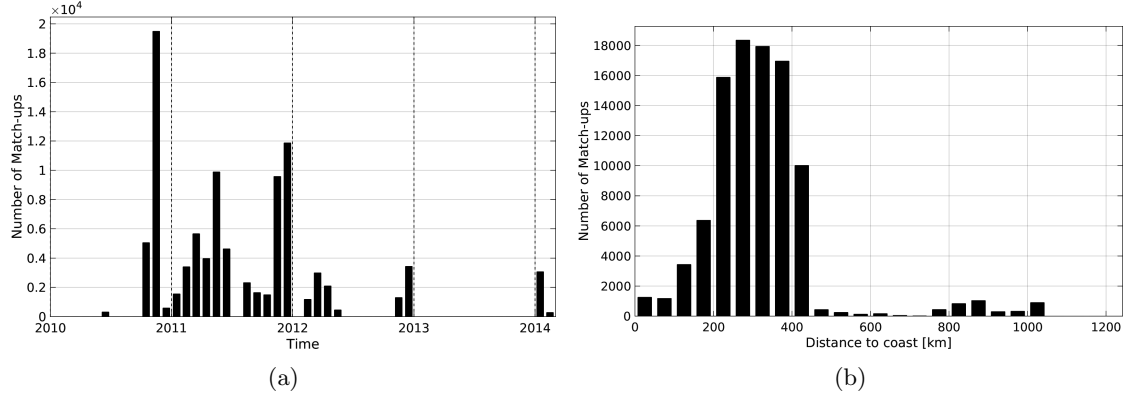
Figure 1: Number of match-ups between TSG-SAMOS and SMOS-L3-ICDC-V3-MONTHLY-0.5DEG SSS as a function of time (a) and as function of the distance to coast (b) over the Southern Ocean Pi-MEP region and for the full satellite product period.
