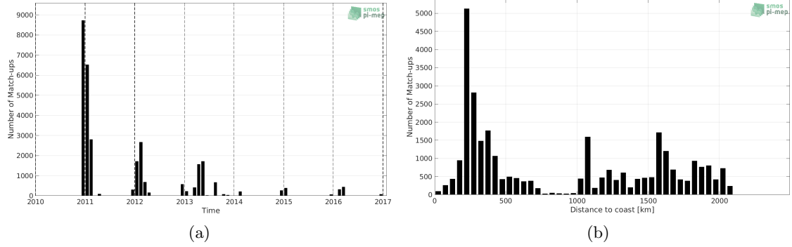
Figure 1: Number of match-ups between TSG (Polarstern) and SMOS SSS L3 v3 Monthly (ICDC) SSS as a function of time (a) and as function of the distance to coast (b) over the Southern Ocean Pi-MEP region and for the full satellite product period.
