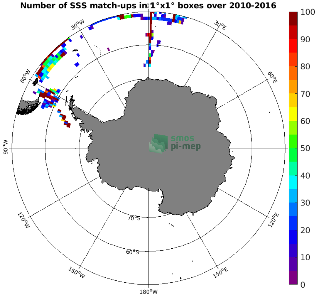
Figure 4: Number of SSS match-ups between TSG (Polarstern) SSS and the SMOS SSS L3 v3 Monthly (ICDC) SSS product for the Southern Ocean Pi-MEP region over 1^\circ \times 1^\circ boxes and for the full satellite product period.
