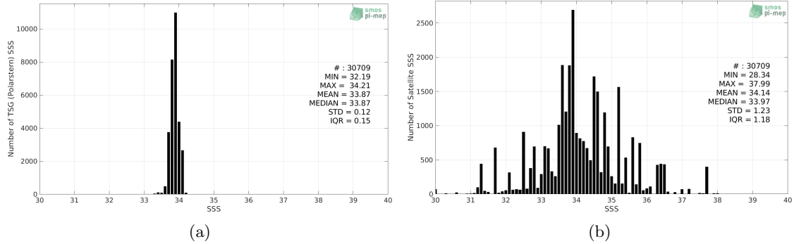
Figure 2: Histograms of SSS from TSG (Polarstern) (a) and SMOS SSS L3 v3 Monthly (ICDC) (b) considering all match-up pairs per bins of 0.1 over the Southern Ocean Pi-MEP region and for the full satellite product period.
