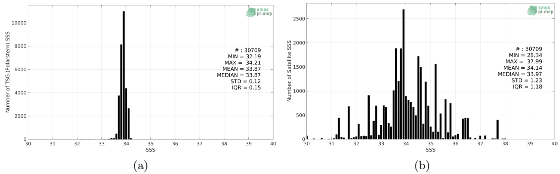
Figure 2: Histograms of SSS from TSG (Polarstern) (a) and SMOS SSS L3 v3 Monthly (ICDC) (b) considering all match-up pairs per bins of 0.1 over the Southern Ocean Pi-MEP region and for the full satellite product period.
