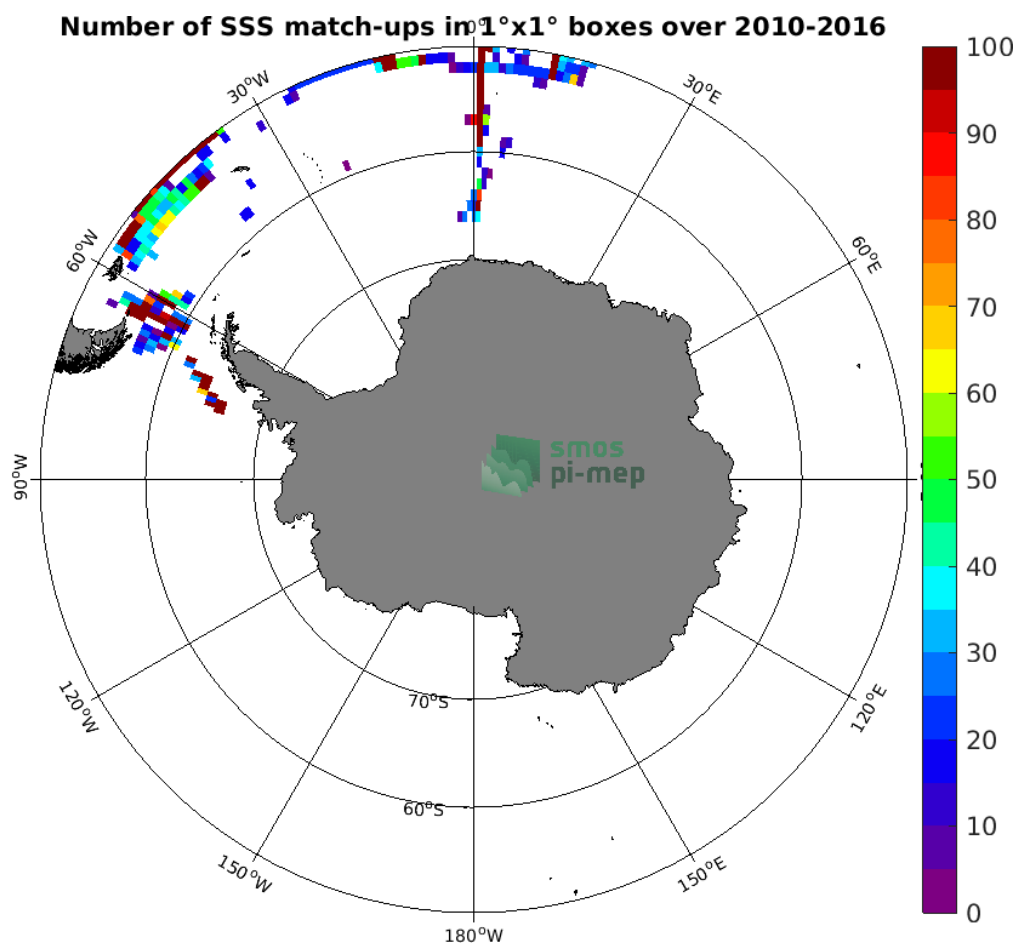
Figure 4: Number of SSS match-ups between TSG (Polarstern) SSS and the SMOS SSS L3 v3 Monthly (ICDC) SSS product for the Southern Ocean Pi-MEP region over 1^\circ \times 1^\circ boxes and for the full satellite product period.
