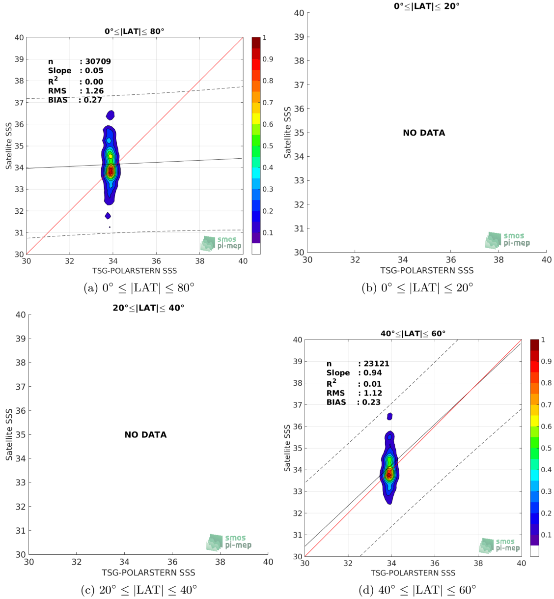
Figure 9: Contour maps of the concentration of SMOS-L3-ICDC-V3-MONTHLY-0.5DEG SSS (y-axis) versus TSG-POLARSTERN SSS (x-axis) at match-up pairs for different latitude bands. For each plot, the red line shows x=y . The black thin and dashed lines indicate a linear fit through the data cloud and the \pm 95\% confidence levels, respectively. The number match-up pairs n , the slope and R^2 coefficient of the linear fit, the root mean square (RMS) and the mean bias between satellite and in situ data are indicated for each latitude band in each plots.
