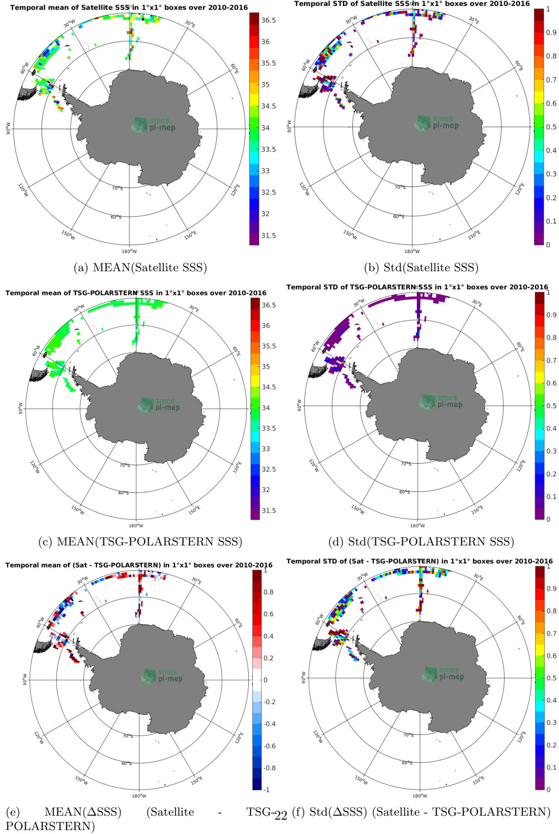
Figure 6: Temporal mean (left) and Std (right) of SSS from SMOS-L3-ICDC-V3-MONTHLY-0.5DEG (top), TSG-POLARSTERN (middle), and of \Delta SSS (Satellite - TSG-POLARSTERN). Only match-up pairs are used to generate these maps.
