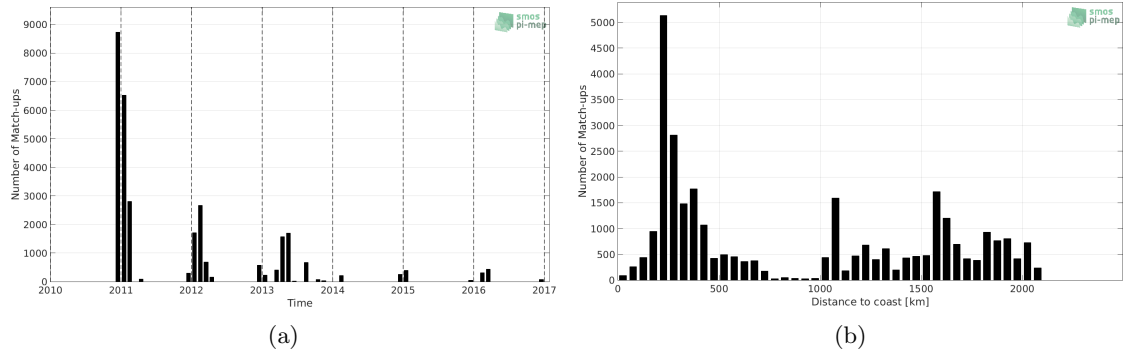
Figure 1: Number of match-ups between TSG-POLARSTERN and SMOS-L3-ICDC-V3-MONTHLY-0.5DEG SSS as a function of time (a) and as function of the distance to coast (b) over the Southern Ocean Pi-MEP region and for the full satellite product period.
