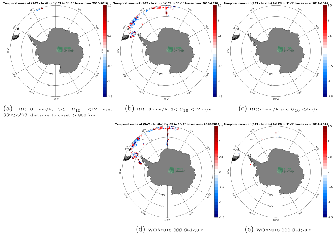
Figure 12: Temporal mean gridded over spatial boxes of size 1^\circ \times 1^\circ of \Delta SSS (SMOS-L3-ICDC-V3-MONTHLY-0.5DEG - TSG-POLARSTERN) for 5 different subdatasets corresponding to: RR=0 mm/h, 3 < U_{10} < 12 m/s, SST > 5^\circ\text{C} , distance to coast > 800 km (a), RR=0 mm/h, 3 < U_{10} < 12 m/s (b), RR > 1 mm/h and U_{10} < 4 m/s (c), WOA2013 SSS Std < 0.2 (d), WOA2013 SSS Std > 0.2 (e).
