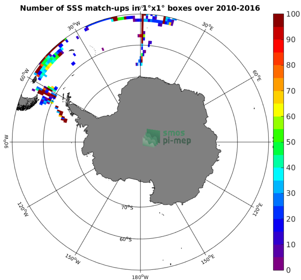
Figure 4: Number of SSS match-ups between TSG-POLARSTERN SSS and the SMOS-L3-ICDC-V3-MONTHLY-0.5DEG SSS product for the Southern Ocean Pi-MEP region over 1^\circ \times 1^\circ boxes and for the full satellite product period.
