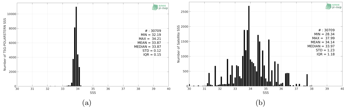
Figure 2: Histograms of SSS from TSG-POLARSTERN (a) and SMOS-L3-ICDC-V3-MONTHLY-0.5DEG (b) considering all match-up pairs per bins of 0.1 over the Southern Ocean Pi-MEP region and for the full satellite product period.
