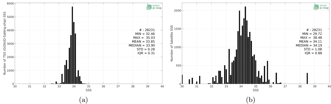
Figure 2: Histograms of SSS from TSG (GOSUD-Sailing-ship) (a) and SMOS SSS L3 v3 Monthly (ICDC) (b) considering all match-up pairs per bins of 0.1 over the Southern Ocean Pi-MEP region and for the full satellite product period.
