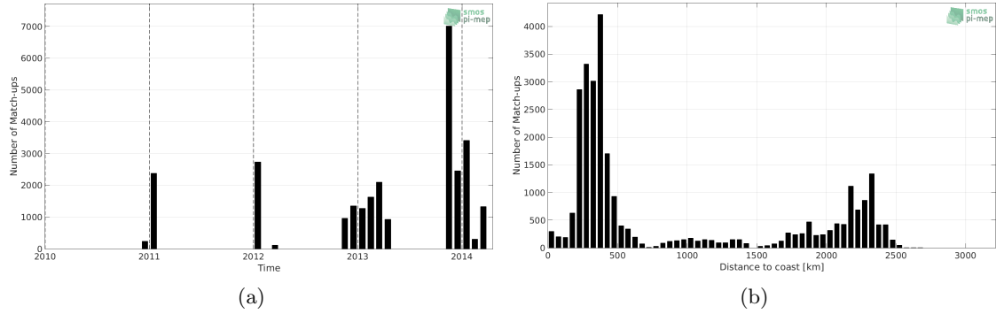
Figure 1: Number of match-ups between TSG (GOSUD-Sailing-ship) and SMOS SSS L3 v3 Monthly (ICDC) SSS as a function of time (a) and as function of the distance to coast (b) over the Southern Ocean Pi-MEP region and for the full satellite product period.
