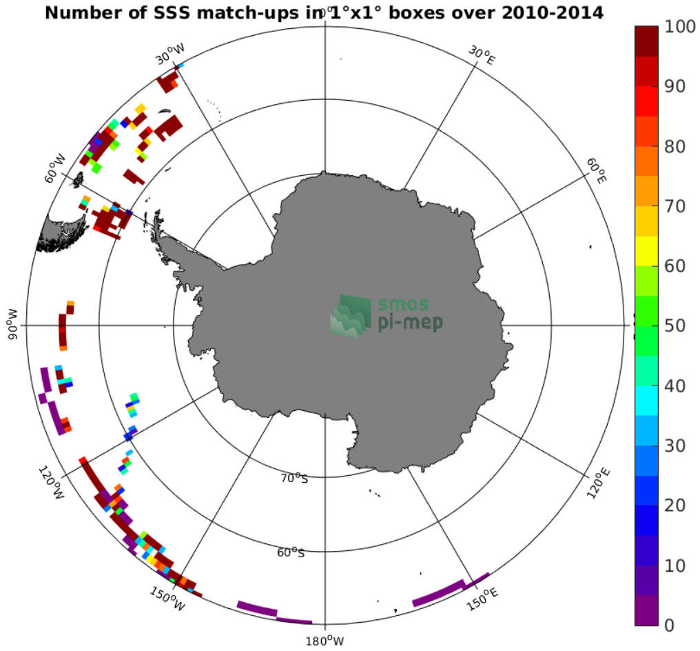
Figure 4: Number of SSS match-ups between TSG (GOSUD-Sailing-ship) SSS and the SMOS SSS L3 v3 Monthly (ICDC) SSS product for the Southern Ocean Pi-MEP region over 1^\circ \times 1^\circ boxes and for the full satellite product period.
