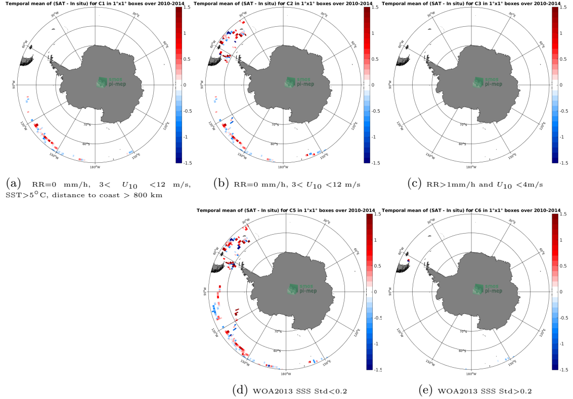
Figure 12: Temporal mean gridded over spatial boxes of size 1°x1° of \Delta\text{SSS} (SMOS SSS L3 v3 Monthly (ICDC) - TSG (GOSUD-Sailing-ship)) for 5 different subdatasets corresponding to: RR=0 mm/h, 3 < U_{10} < 12 m/s, SST > 5^\circ\text{C} , distance to coast > 800 km (a), RR=0 mm/h, 3 < U_{10} < 12 m/s (b), RR > 1 mm/h and U_{10} < 4 m/s (c), WOA2013 SSS Std < 0.2 (d), WOA2013 SSS Std > 0.2 (e).
