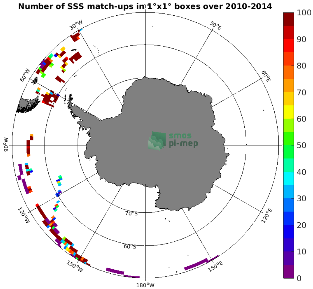
Figure 4: Number of SSS match-ups between TSG (GOSUD-Sailing-ship) SSS and the SMOS SSS L3 v3 Monthly (ICDC) SSS product for the Southern Ocean Pi-MEP region over 1^\circ \times 1^\circ boxes and for the full satellite product period.
