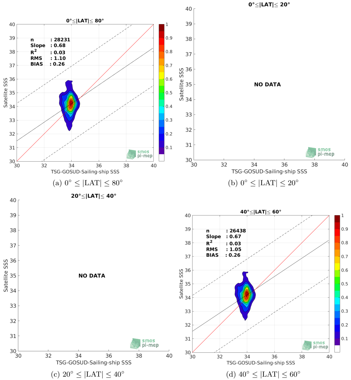
Figure 9: Contour maps of the concentration of SMOS-L3-ICDC-V3-MONTHLY-0.5DEG SSS (y-axis) versus TSG-GOSUD-Sailing-ship SSS (x-axis) at match-up pairs for different latitude bands. For each plot, the red line shows x=y . The black thin and dashed lines indicate a linear fit through the data cloud and the \pm 95\% confidence levels, respectively. The number match-up pairs n , the slope and R^2 coefficient of the linear fit, the root mean square (RMS) and the mean bias between satellite and in situ data are indicated for each latitude band in each plots.
