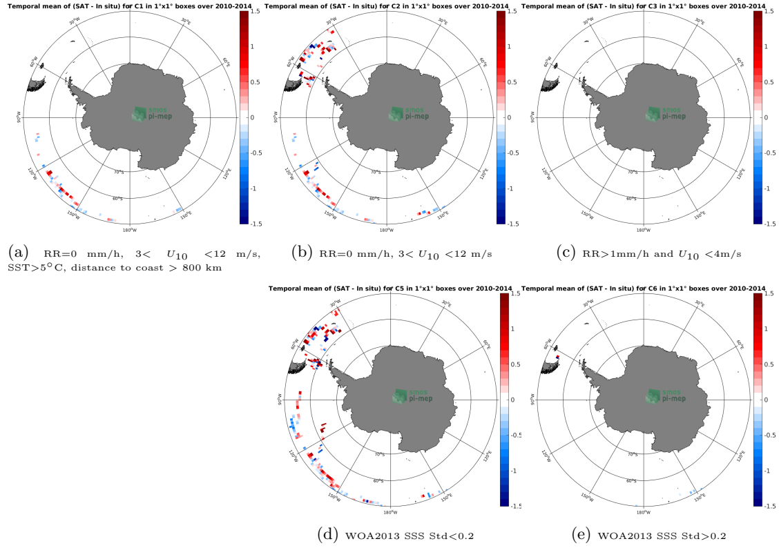
Figure 12: Temporal mean gridded over spatial boxes of size 1^\circ \times 1^\circ of \Delta SSS (SMOS-L3-ICDC-V3-MONTHLY-0.5DEG - TSG-GOSUD-Sailing-ship) for 5 different subdatasets corresponding to: RR=0 mm/h, 3 < U_{10} < 12 m/s, SST > 5^\circ\text{C} , distance to coast > 800 km (a), RR=0 mm/h, 3 < U_{10} < 12 m/s (b), RR > 1 mm/h and U_{10} < 4 m/s (c), WOA2013 SSS Std < 0.2 (d), WOA2013 SSS Std > 0.2 (e).
