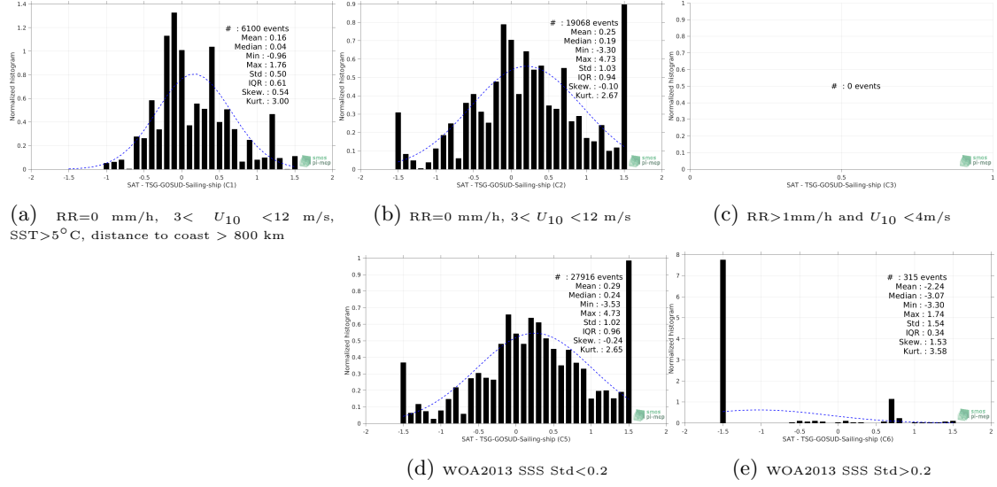
Figure 13: Normalized histogram of \Delta SSS (SMOS-L3-ICDC-V3-MONTHLY-0.5DEG - TSG-GOSUD-Sailing-ship) for 5 different subdatasets corresponding to: RR=0 mm/h, 3 < U_{10} < 12 m/s, SST>5°C, distance to coast > 800 km (a), RR=0 mm/h, 3 < U_{10} < 12 m/s (b), RR>1mm/h and U_{10} < 4 m/s (c), WOA2013 SSS Std<0.2 (d), WOA2013 SSS Std>0.2 (e).
