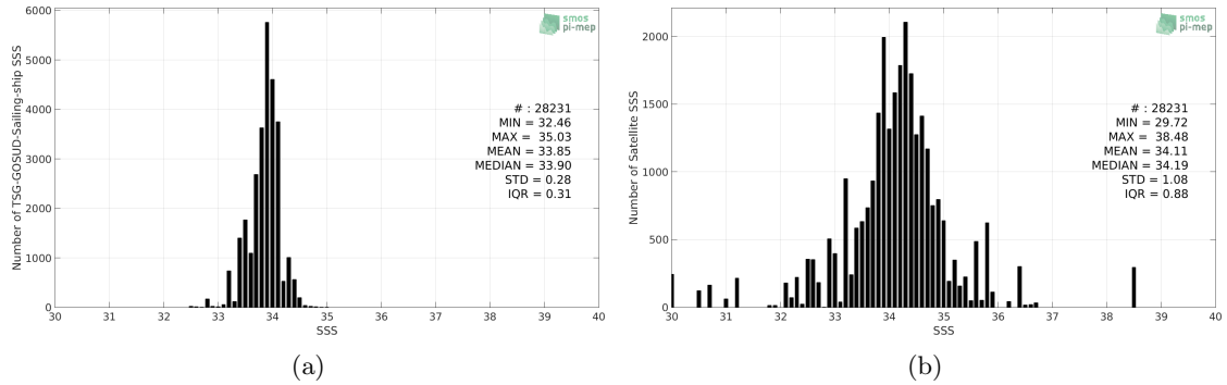
Figure 2: Histograms of SSS from TSG-GOSUD-Sailing-ship (a) and SMOS-L3-ICDC-V3-MONTHLY-0.5DEG (b) considering all match-up pairs per bins of 0.1 over the Southern Ocean Pi-MEP region and for the full satellite product period.
