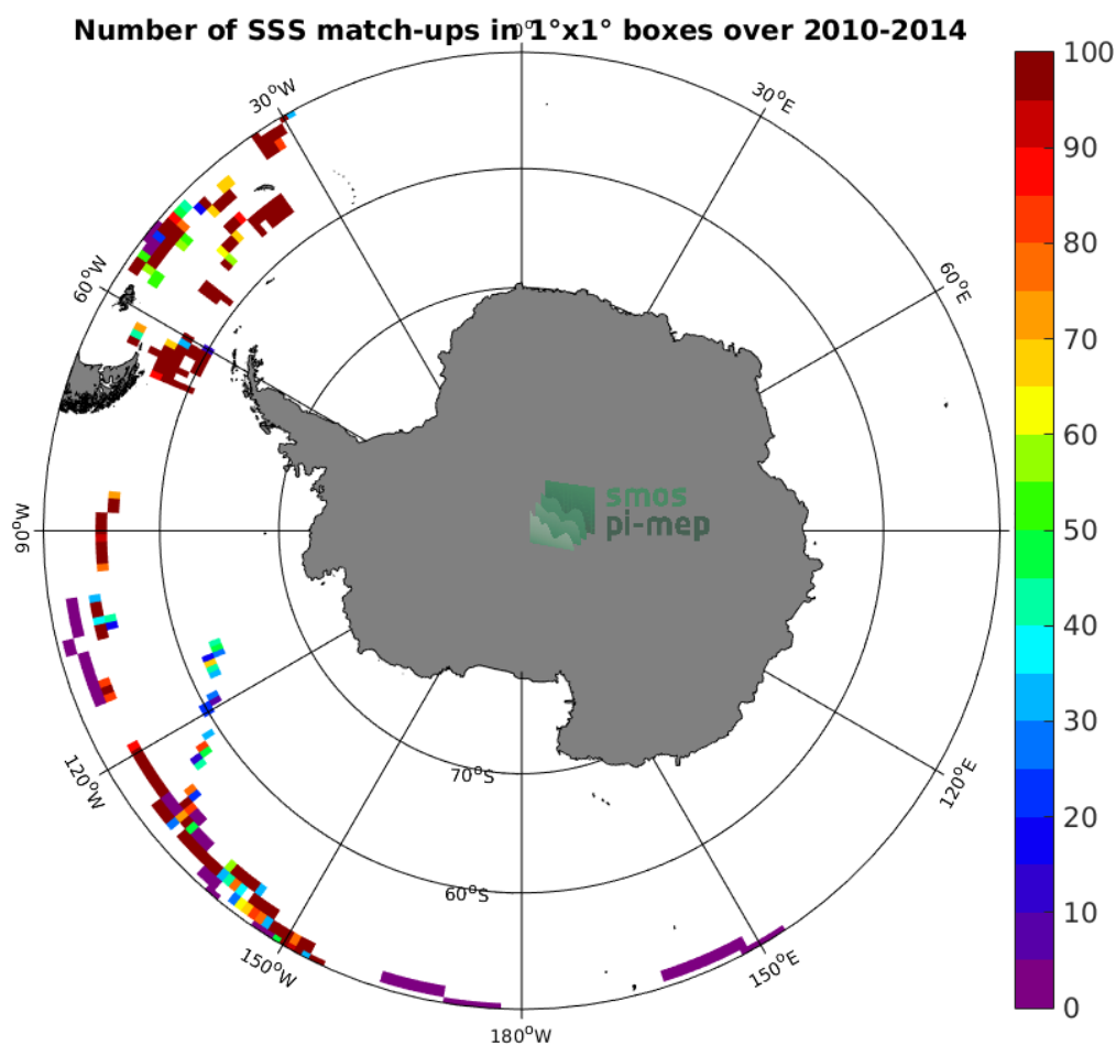
Figure 4: Number of SSS match-ups between TSG-GOSUD-Sailing-ship SSS and the SMOS-L3-ICDC-V3-MONTHLY-0.5DEG SSS product for the Southern Ocean Pi-MEP region over 1^\circ \times 1^\circ boxes and for the full satellite product period.
