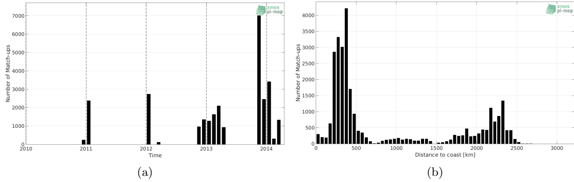
Figure 1: Number of match-ups between TSG-GOSUD-Sailing-ship and SMOS-L3-ICDC-V3-MONTHLY-0.5DEG SSS as a function of time (a) and as function of the distance to coast (b) over the Southern Ocean Pi-MEP region and for the full satellite product period.
