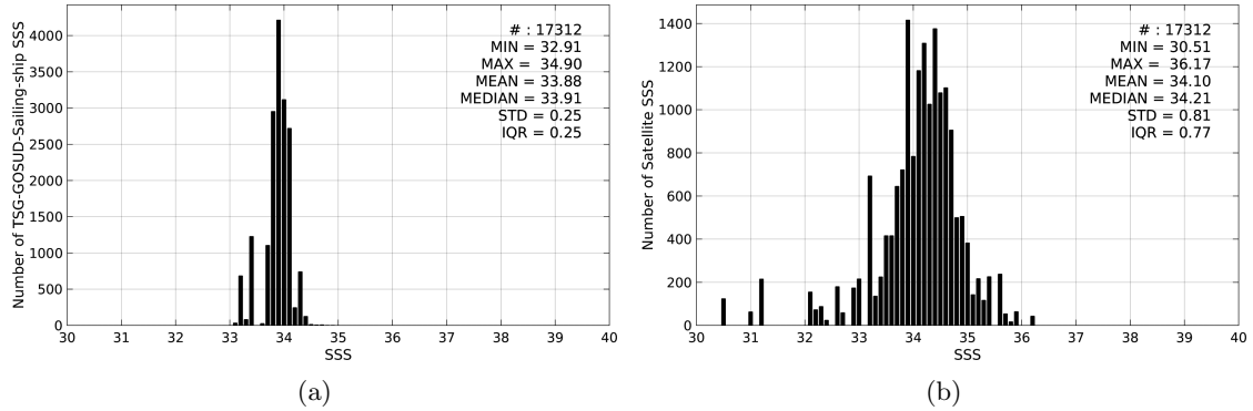
Figure 2: Histograms of SSS from TSG-GOSUD-Sailing-ship (a) and SMOS-L3-ICDC-V3-MONTHLY-0.5DEG (b) considering all match-up pairs per bins of 0.1 over the Southern Ocean Pi-MEP region and for the full satellite product period.
