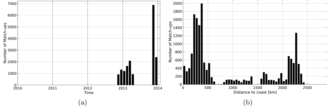
Figure 1: Number of match-ups between TSG-GOSUD-Sailing-ship and SMOS-L3-ICDC-V3-MONTHLY-0.5DEG SSS as a function of time (a) and as function of the distance to coast (b) over the Southern Ocean Pi-MEP region and for the full satellite product period.
