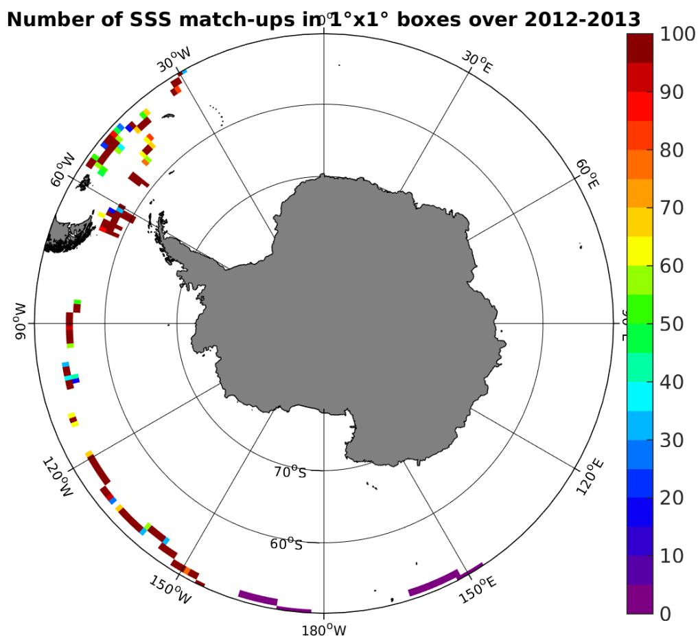
Figure 4: Number of SSS match-ups between TSG-GOSUD-Sailing-ship SSS and the SMOS-L3-ICDC-V3-MONTHLY-0.5DEG SSS product for the Southern Ocean Pi-MEP region over 1^\circ \times 1^\circ boxes and for the full satellite product period.
