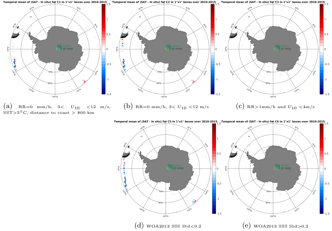
Figure 12: Temporal mean gridded over spatial boxes of size 1^{\circ}\times 1^{\circ} of \Delta\text{SSS} (SMOS SSS L3 v3 Monthly (ICDC) - TSG (GOSUD-Research-vessel)) for 5 different subdatasets corresponding to: RR=0 mm/h, 3 < U_{10} < 12 m/s, SST >5^{\circ}\text{C} , distance to coast > 800 km (a), RR=0 mm/h, 3 < U_{10} < 12 m/s (b), RR>1 mm/h and U_{10} < 4 m/s (c), WOA2013 SSS Std <0.2 (d), WOA2013 SSS Std >0.2 (e).
