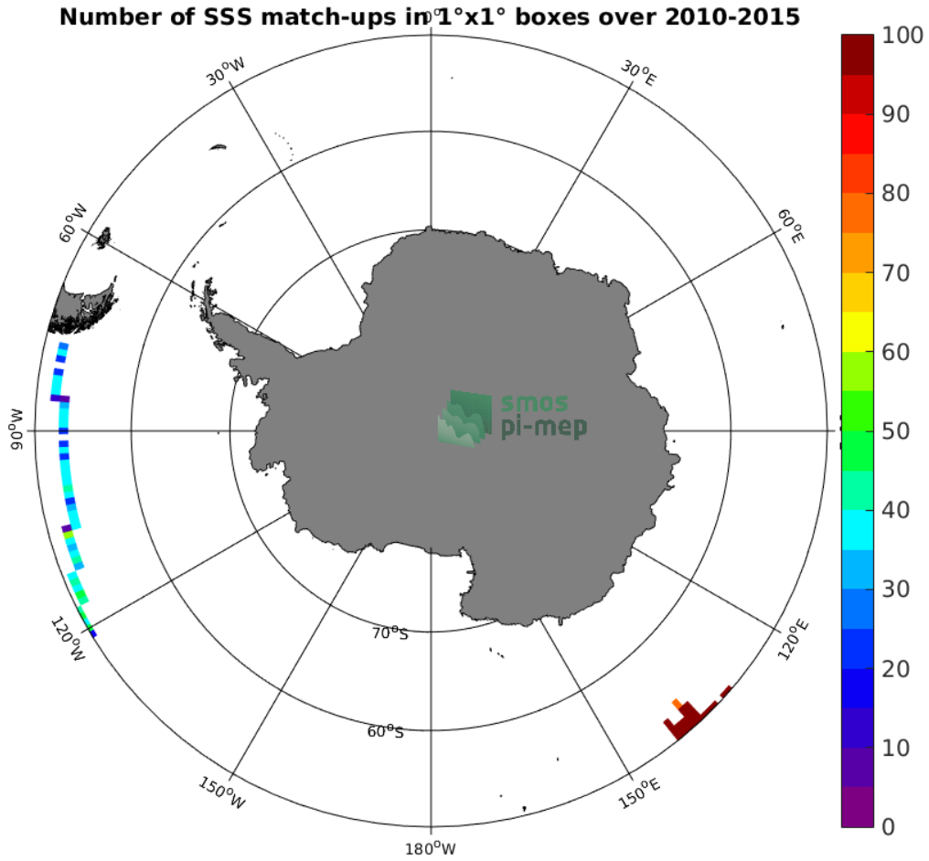
Figure 4: Number of SSS match-ups between TSG (GOSUD-Research-vessel) SSS and the SMOS SSS L3 v3 Monthly (ICDC) SSS product for the Southern Ocean Pi-MEP region over 1^\circ \times 1^\circ boxes and for the full satellite product period.
