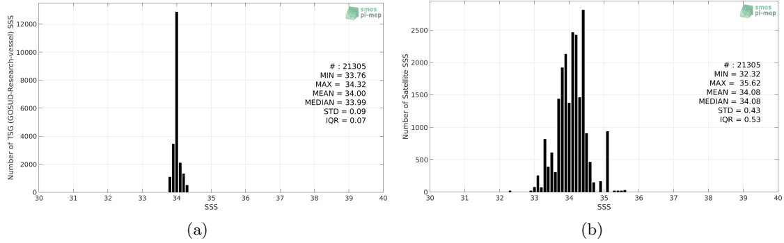
Figure 2: Histograms of SSS from TSG (GOSUD-Research-vessel) (a) and SMOS SSS L3 v3 Monthly (ICDC) (b) considering all match-up pairs per bins of 0.1 over the Southern Ocean Pi-MEP region and for the full satellite product period.
