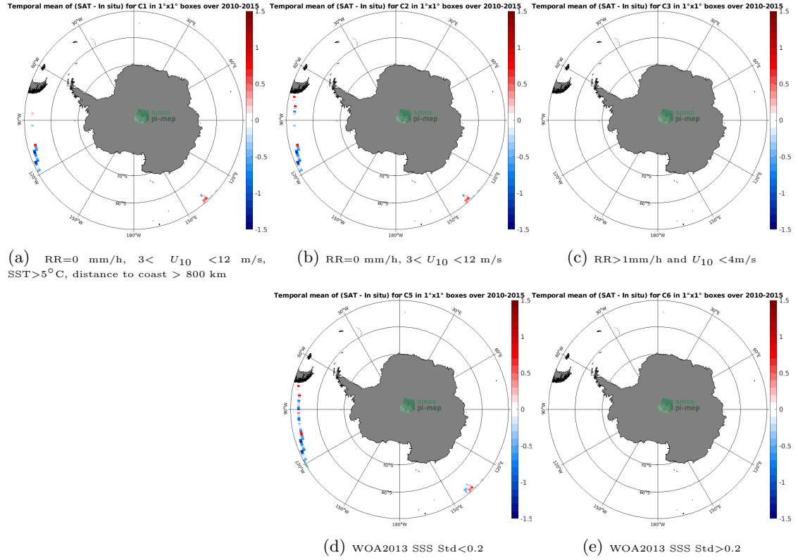
Figure 12: Temporal mean gridded over spatial boxes of size 1°x1° of \Delta SSS (SMOS SSS L3 v3 Monthly (ICDC) - TSG (GOSUD-Research-vessel)) for 5 different subdatasets corresponding to: RR=0 mm/h, 3 < U_{10} < 12 m/s, SST>5°C, distance to coast > 800 km (a), RR=0 mm/h, 3 < U_{10} < 12 m/s (b), RR>1mm/h and U_{10} < 4 m/s (c), WOA2013 SSS Std<0.2 (d), WOA2013 SSS Std>0.2 (e).
