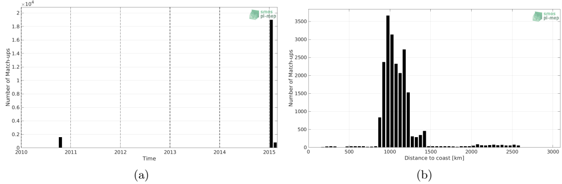
Figure 1: Number of match-ups between TSG (GOSUD-Research-vessel) and SMOS SSS L3 v3 Monthly (ICDC) SSS as a function of time (a) and as function of the distance to coast (b) over the Southern Ocean Pi-MEP region and for the full satellite product period.
