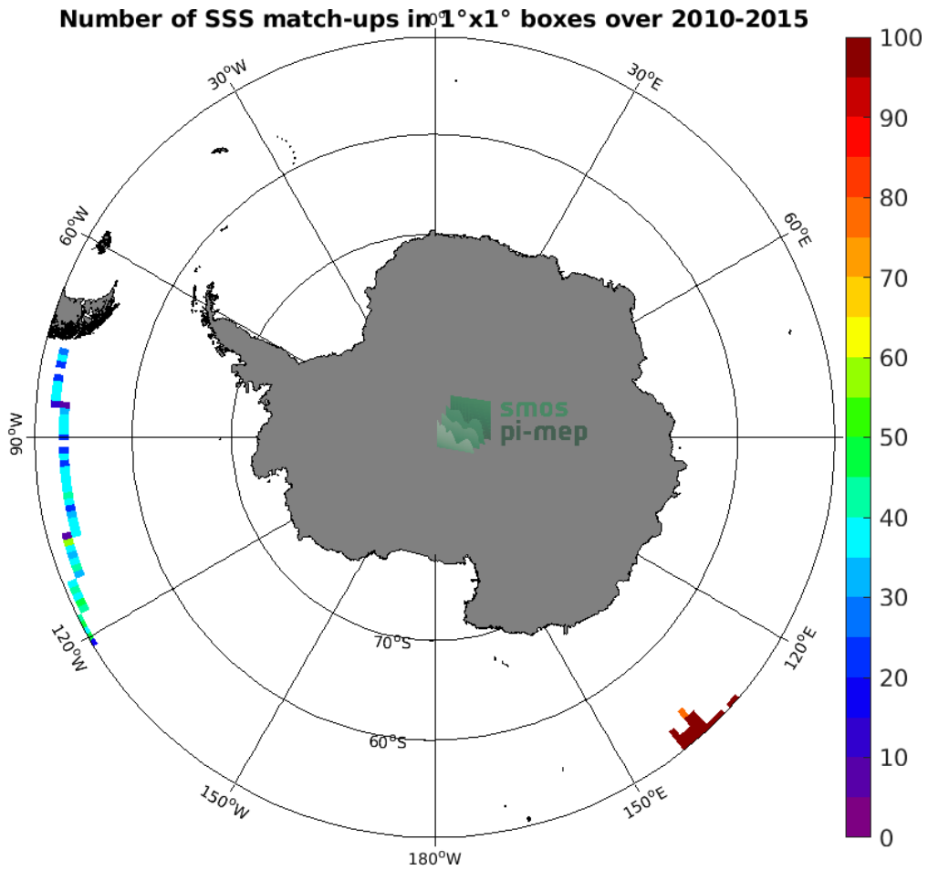
Figure 4: Number of SSS match-ups between TSG (GOSUD-Research-vessel) SSS and the SMOS SSS L3 v3 Monthly (ICDC) SSS product for the Southern Ocean Pi-MEP region over 1^\circ \times 1^\circ boxes and for the full satellite product period.
