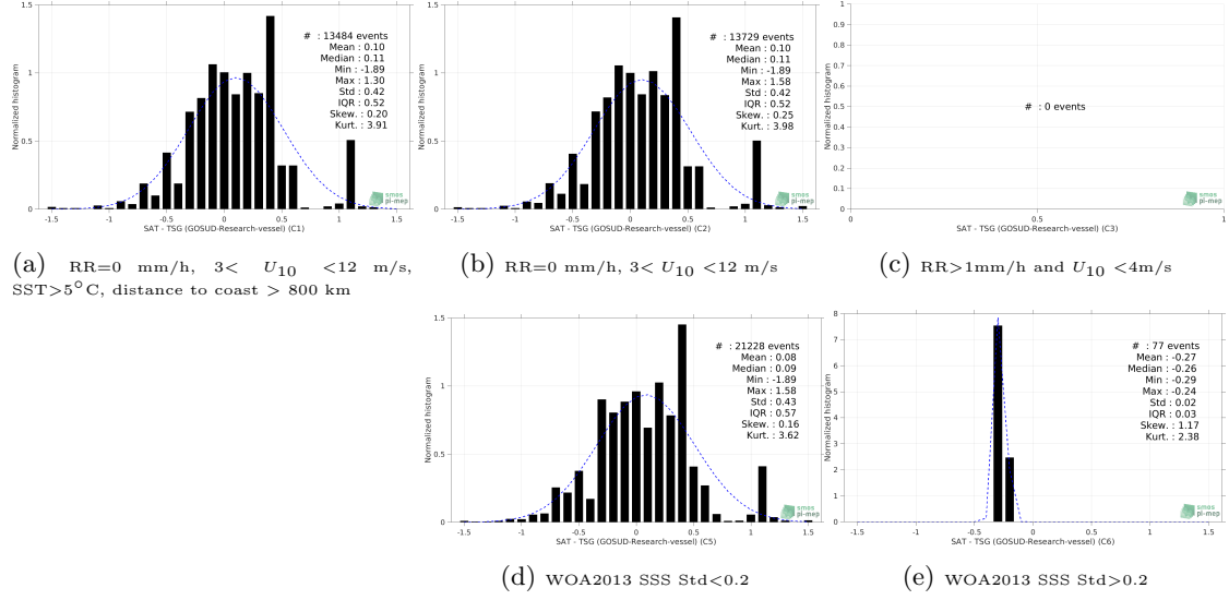
Figure 13: Normalized histogram of \Delta\text{SSS} (SMOS SSS L3 v3 Monthly (ICDC) - TSG (GOSUD-Research-vessel)) for 5 different subdatasets corresponding to: RR=0 mm/h, 3 < U_{10} < 12 m/s, SST > 5^\circ\text{C} , distance to coast > 800 km (a), RR=0 mm/h, 3 < U_{10} < 12 m/s (b), RR > 1 mm/h and U_{10} < 4 m/s (c), WOA2013 SSS Std < 0.2 (d), WOA2013 SSS Std > 0.2 (e).
