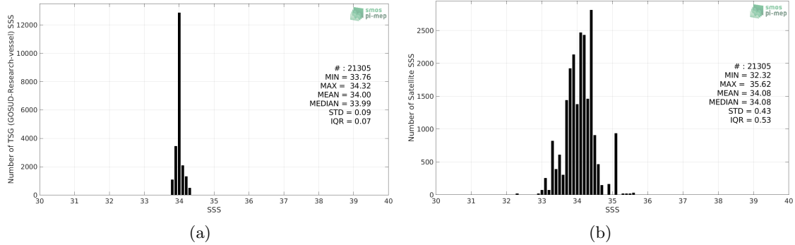
Figure 2: Histograms of SSS from TSG (GOSUD-Research-vessel) (a) and SMOS SSS L3 v3 Monthly (ICDC) (b) considering all match-up pairs per bins of 0.1 over the Southern Ocean Pi-MEP region and for the full satellite product period.
