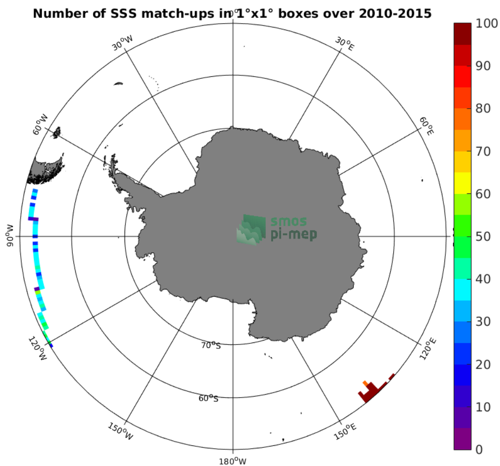
Figure 4: Number of SSS match-ups between TSG-GOSUD-Research-vessel SSS and the SMOS-L3-ICDC-V3-MONTHLY-0.5DEG SSS product for the Southern Ocean Pi-MEP region over 1^\circ \times 1^\circ boxes and for the full satellite product period.
