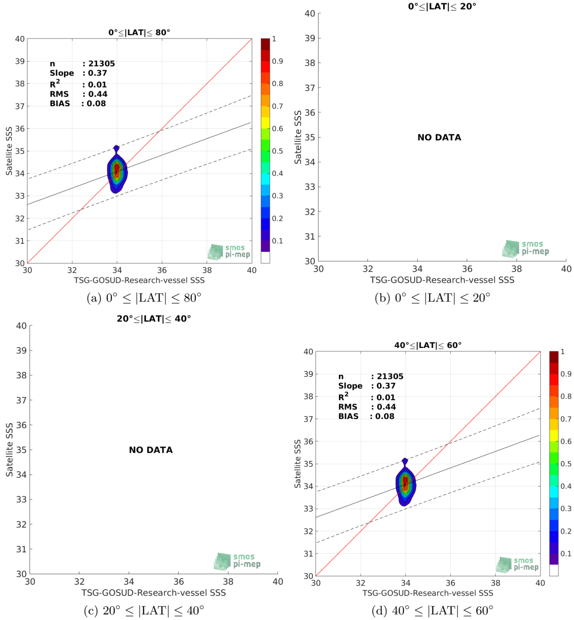
Figure 9: Contour maps of the concentration of SMOS-L3-ICDC-V3-MONTHLY-0.5DEG SSS (y-axis) versus TSG-GOSUD-Research-vessel SSS (x-axis) at match-up pairs for different latitude bands. For each plot, the red line shows x=y . The black thin and dashed lines indicate a linear fit through the data cloud and the \pm 95\% confidence levels, respectively. The number match-up pairs n , the slope and R^2 coefficient of the linear fit, the root mean square (RMS) and the mean bias between satellite and in situ data are indicated for each latitude band in each plots.
