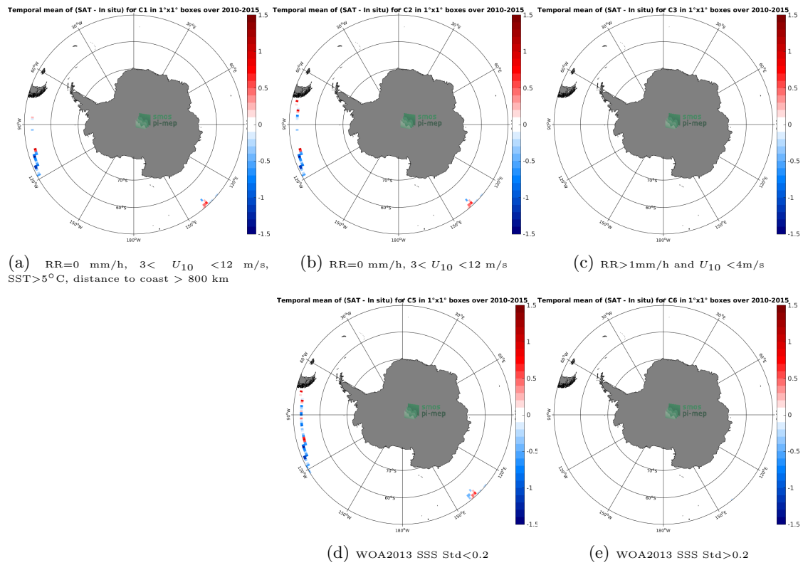
Figure 12: Temporal mean gridded over spatial boxes of size 1^\circ \times 1^\circ of \Delta SSS (SMOS-L3-ICDC-V3-MONTHLY-0.5DEG - TSG-GOSUD-Research-vessel) for 5 different subdatasets corresponding to: RR=0 mm/h, 3 < U_{10} < 12 m/s, SST >5^\circ\text{C} , distance to coast > 800 km (a), RR=0 mm/h, 3 < U_{10} < 12 m/s (b), RR >1 mm/h and U_{10} < 4 m/s (c), WOA2013 SSS Std <0.2 (d), WOA2013 SSS Std >0.2 (e).
