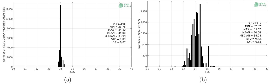
Figure 2: Histograms of SSS from TSG-GOSUD-Research-vessel (a) and SMOS-L3-ICDC-V3-MONTHLY-0.5DEG (b) considering all match-up pairs per bins of 0.1 over the Southern Ocean Pi-MEP region and for the full satellite product period.
