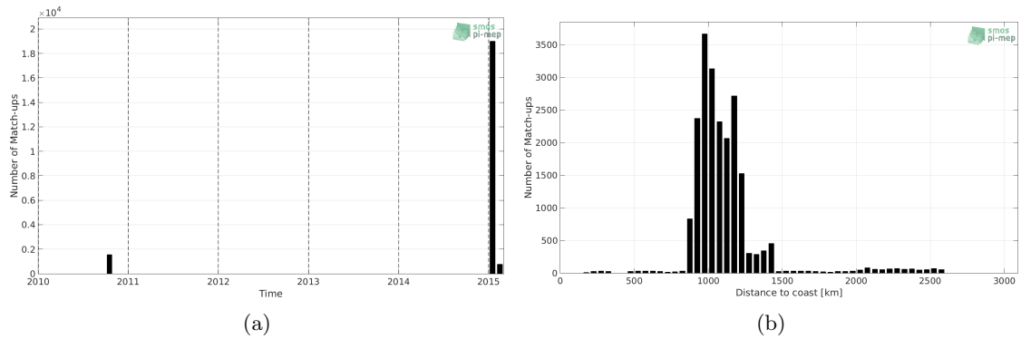
Figure 1: Number of match-ups between TSG-GOSUD-Research-vessel and SMOS-L3-ICDC-V3-MONTHLY-0.5DEG SSS as a function of time (a) and as function of the distance to coast (b) over the Southern Ocean Pi-MEP region and for the full satellite product period.
