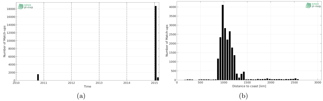
Figure 1: Number of match-ups between TSG-GOSUD-Research-vessel and SMOS-L3-ICDC-V3-MONTHLY-0.5DEG SSS as a function of time (a) and as function of the distance to coast (b) over the Southern Ocean Pi-MEP region and for the full satellite product period.
