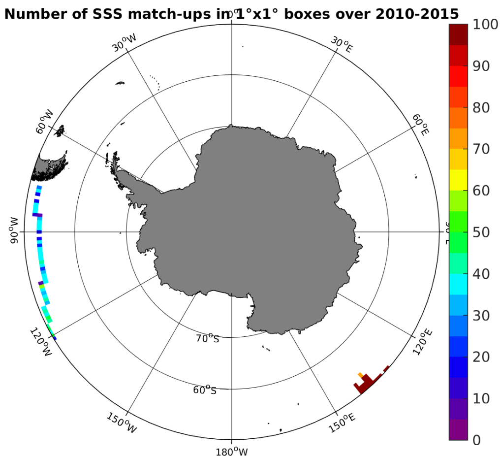
Figure 4: Number of SSS match-ups between TSG-GOSUD-Research-vessel SSS and the SMOS-L3-ICDC-V3-MONTHLY-0.5DEG SSS product for the Southern Ocean Pi-MEP region over 1^\circ \times 1^\circ boxes and for the full satellite product period.
