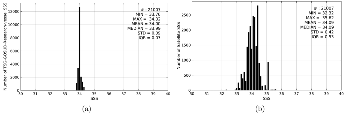
Figure 2: Histograms of SSS from TSG-GOSUD-Research-vessel (a) and SMOS-L3-ICDC-V3-MONTHLY-0.5DEG (b) considering all match-up pairs per bins of 0.1 over the Southern Ocean Pi-MEP region and for the full satellite product period.
