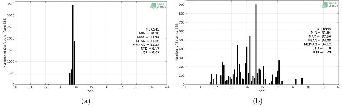
Figure 2: Histograms of SSS from Surface drifters (a) and SMOS SSS L3 v3 Monthly (ICDC) (b) considering all match-up pairs per bins of 0.1 over the Southern Ocean Pi-MEP region and for the full satellite product period.
