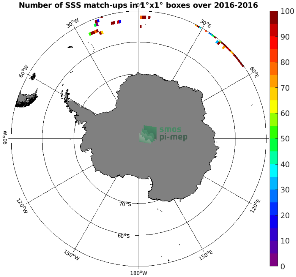
Figure 3: Number of SSS match-ups between Surface drifters SSS and the SMOS SSS L3 v3 Monthly (ICDC) SSS product for the Southern Ocean Pi-MEP region over 1^\circ \times 1^\circ boxes and for the full satellite product period.
