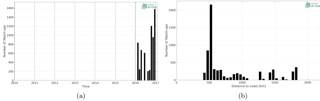
Figure 1: Number of match-ups between Surface drifters and SMOS SSS L3 v3 Monthly (ICDC) SSS as a function of time (a) and as function of the distance to coast (b) over the Southern Ocean Pi-MEP region and for the full satellite product period.
