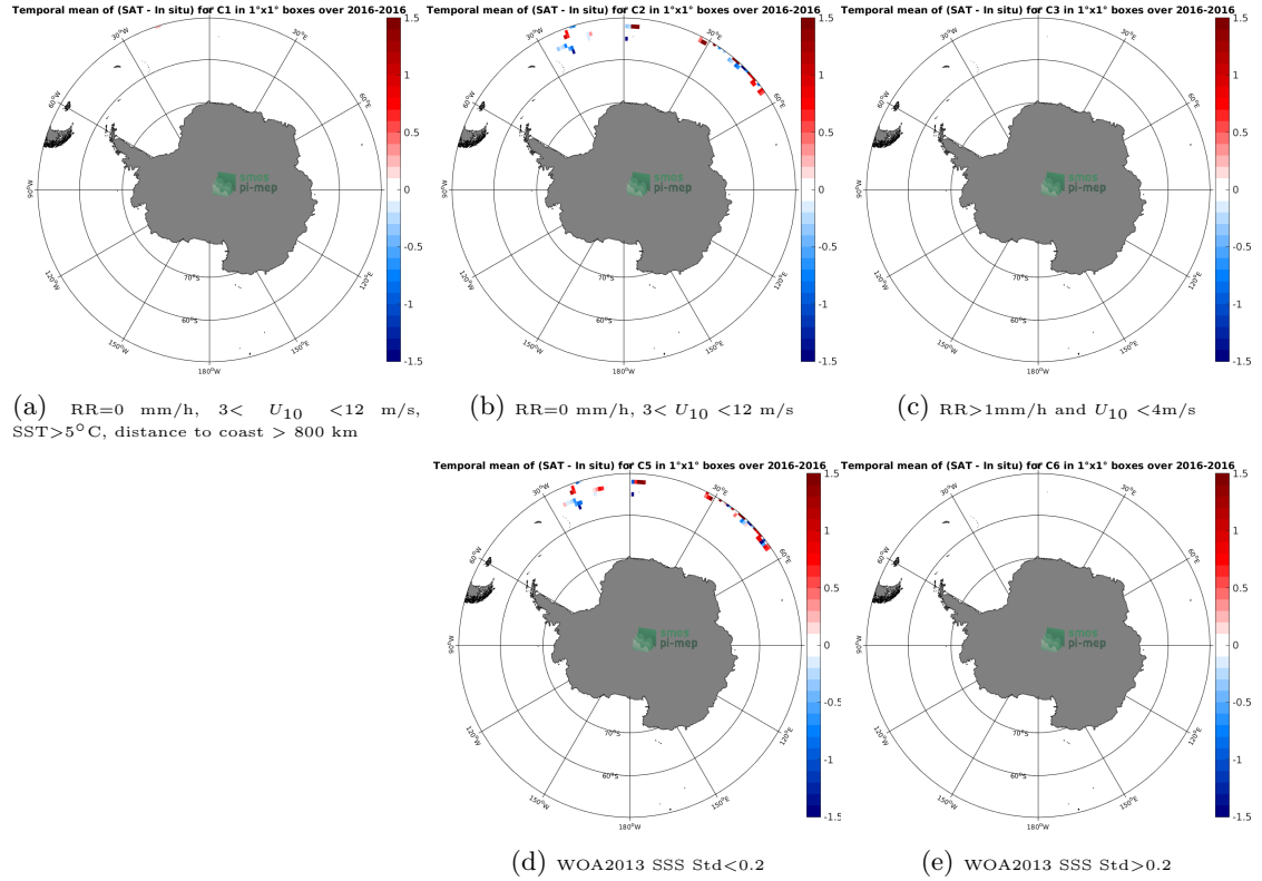
Figure 11: Temporal mean gridded over spatial boxes of size 1^{\circ}\times 1^{\circ} of \Delta\text{SSS} (SMOS-L3-ICDC-V3-MONTHLY-0.5DEG - Surface drifters) for 5 different subdatasets corresponding to:RR=0 mm/h, 3 < U_{10} < 12 m/s, SST >5^{\circ}\text{C} , distance to coast > 800 km (a), RR=0 mm/h, 3 < U_{10} < 12 m/s (b), RR >1 mm/h and U_{10} < 4 m/s (c), WOA2013 SSS Std <0.2 (d), WOA2013 SSS Std >0.2 (e).
