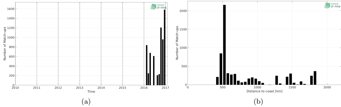
Figure 1: Number of match-ups between Surface drifters and SMOS-L3-ICDC-V3-MONTHLY-0.5DEG SSS as a function of time (a) and as function of the distance to coast (b) over the Southern Ocean Pi-MEP region and for the full satellite product period.
