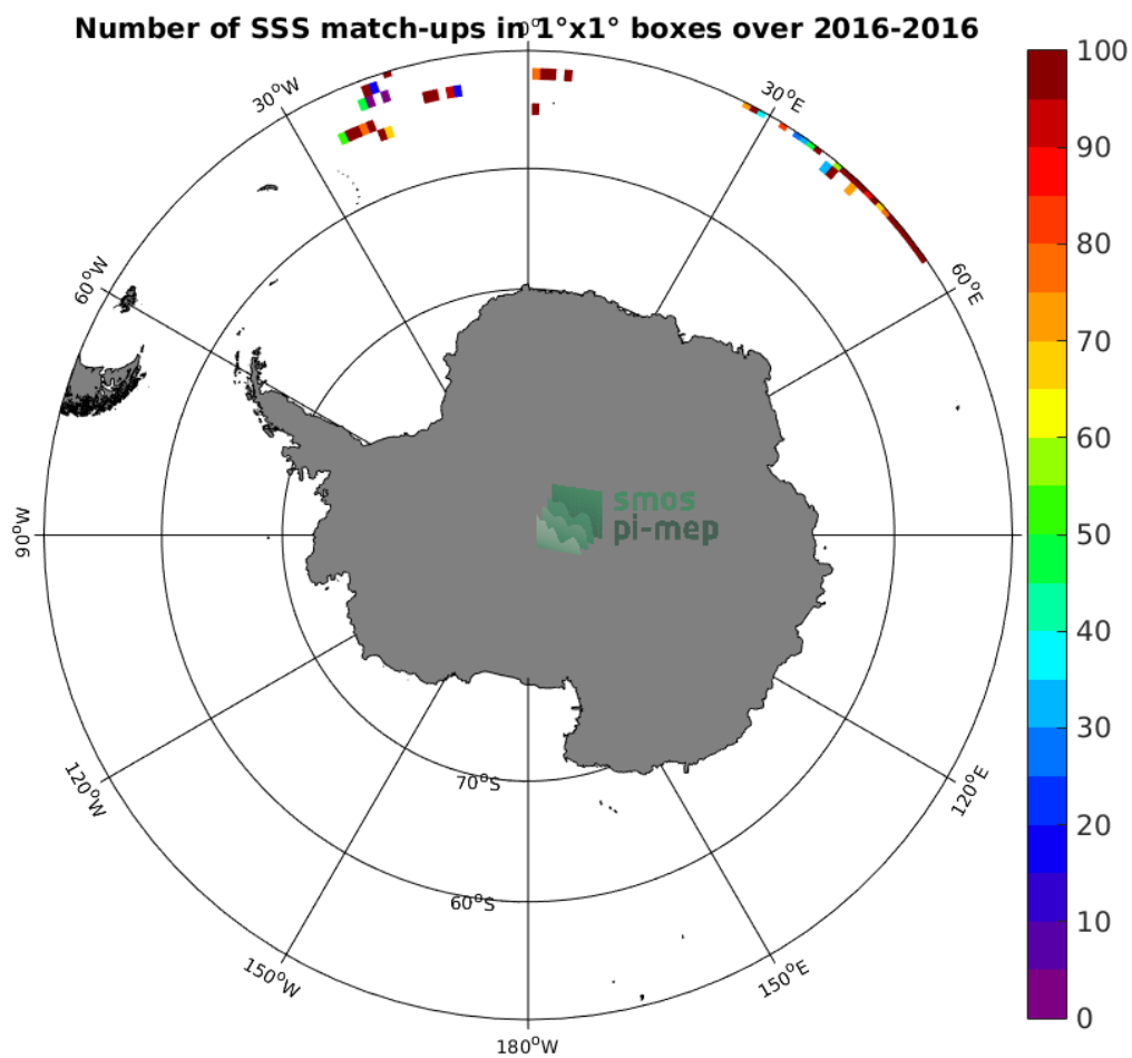
Figure 3: Number of SSS match-ups between Surface drifters SSS and the SMOS-L3-ICDC-V3-MONTHLY-0.5DEG SSS product for the Southern Ocean Pi-MEP region over 1^\circ \times 1^\circ boxes and for the full satellite product period.
