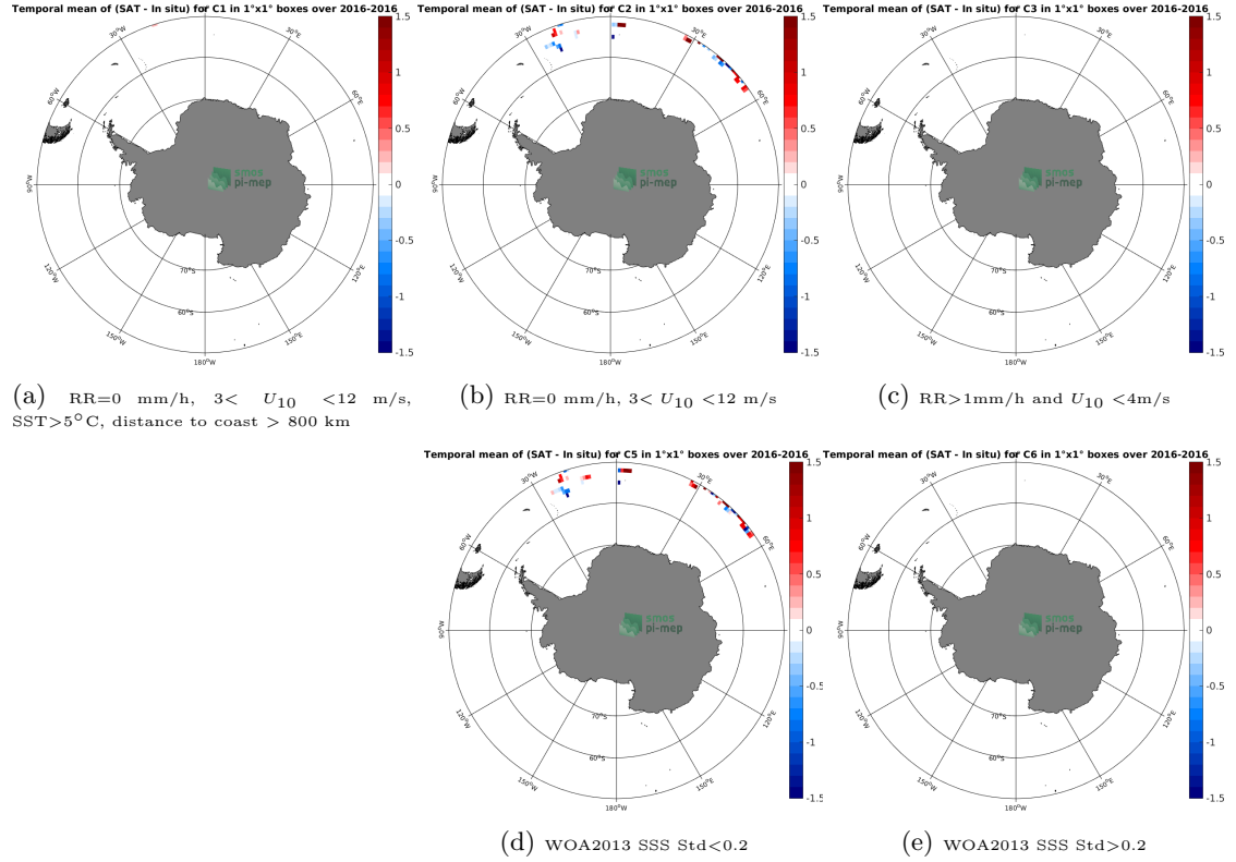
Figure 11: Temporal mean gridded over spatial boxes of size 1^\circ \times 1^\circ of \Delta SSS (SMOS-L3-ICDC-V3-MONTHLY-0.5DEG - Surface drifters) for 5 different subdatasets corresponding to: RR=0 mm/h, 3 < U_{10} < 12 m/s, SST > 5^\circ C , distance to coast > 800 km (a), RR=0 mm/h, 3 < U_{10} < 12 m/s (b), RR > 1 mm/h and U_{10} < 4 m/s (c), WOA2013 SSS Std < 0.2 (d), WOA2013 SSS Std > 0.2 (e).
