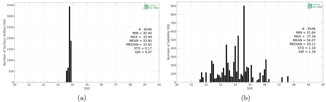
Figure 2: Histograms of SSS from Surface drifters (a) and SMOS-L3-ICDC-V3-MONTHLY-0.5DEG (b) considering all match-up pairs per bins of 0.1 over the Southern Ocean Pi-MEP region and for the full satellite product period.
