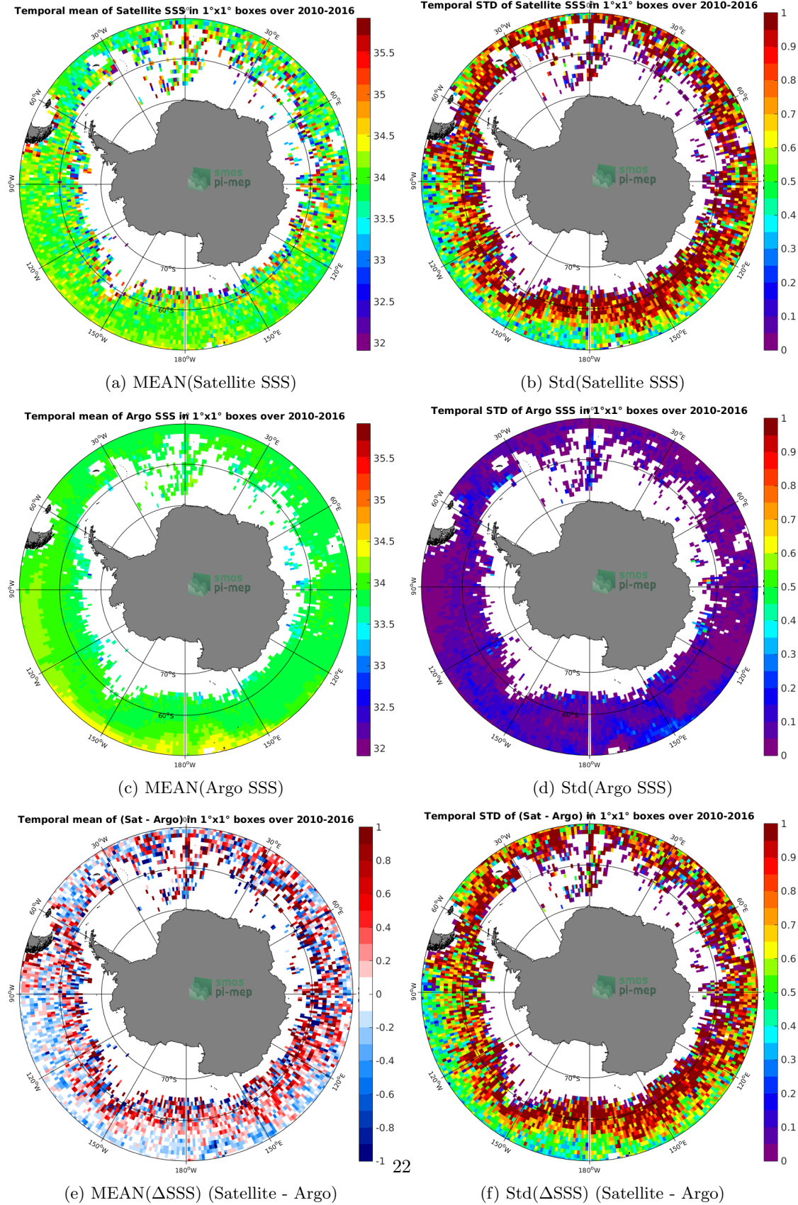
Figure 6: Temporal mean (left) and Std (right) of SSS from SMOS SSS L3 v3 Monthly (ICDC) (top), Argo (middle), and of \Delta SSS (Satellite - Argo). Only match-up pairs are used to generate these maps.
