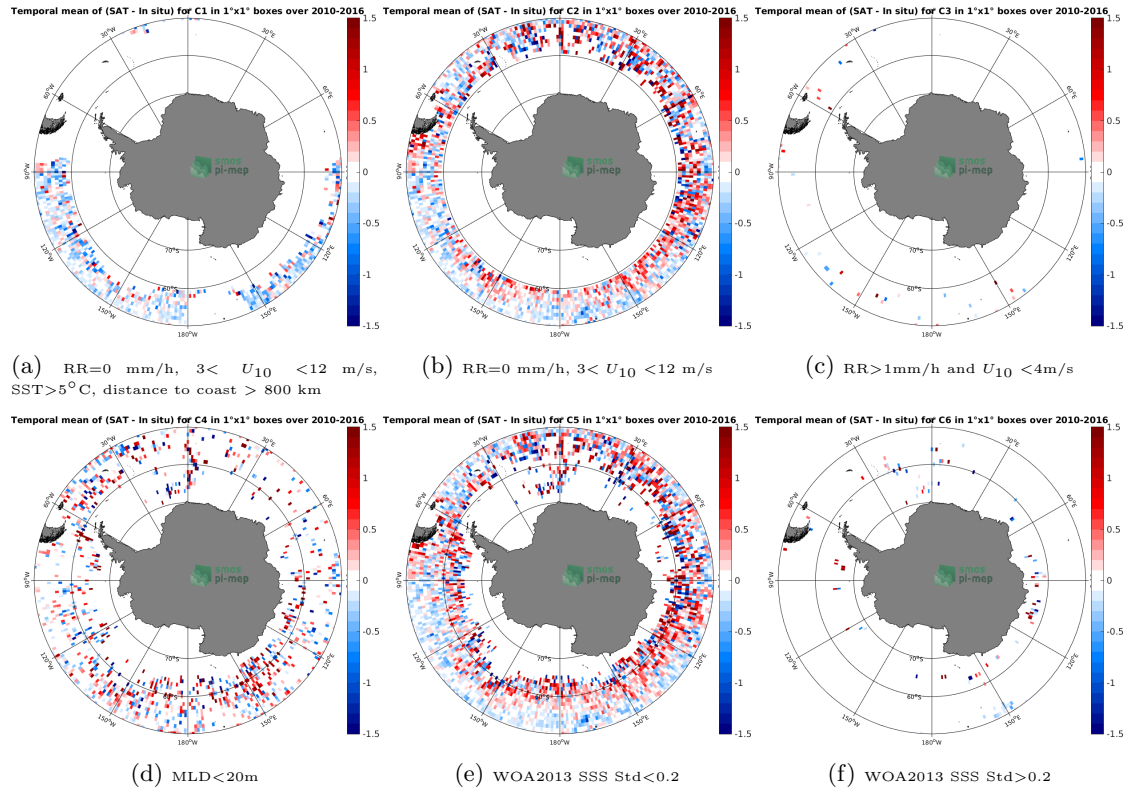
Figure 12: Temporal mean gridded over spatial boxes of size 1^{\circ} \times 1^{\circ} of \Delta\text{SSS} (SMOS SSS L3 v3 Monthly (ICDC) - Argo) for 6 different subdatasets corresponding to: RR=0 mm/h, 3 < U_{10} < 12 m/s, SST >5^{\circ}\text{C} , distance to coast > 800 km (a), RR=0 mm/h, 3 < U_{10} < 12 m/s (b), RR >1 mm/h and U_{10} < 4 m/s (c),MLD <20 m (d),WOA2013 SSS Std <0.2 (e),WOA2013 SSS Std >0.2 (f).
