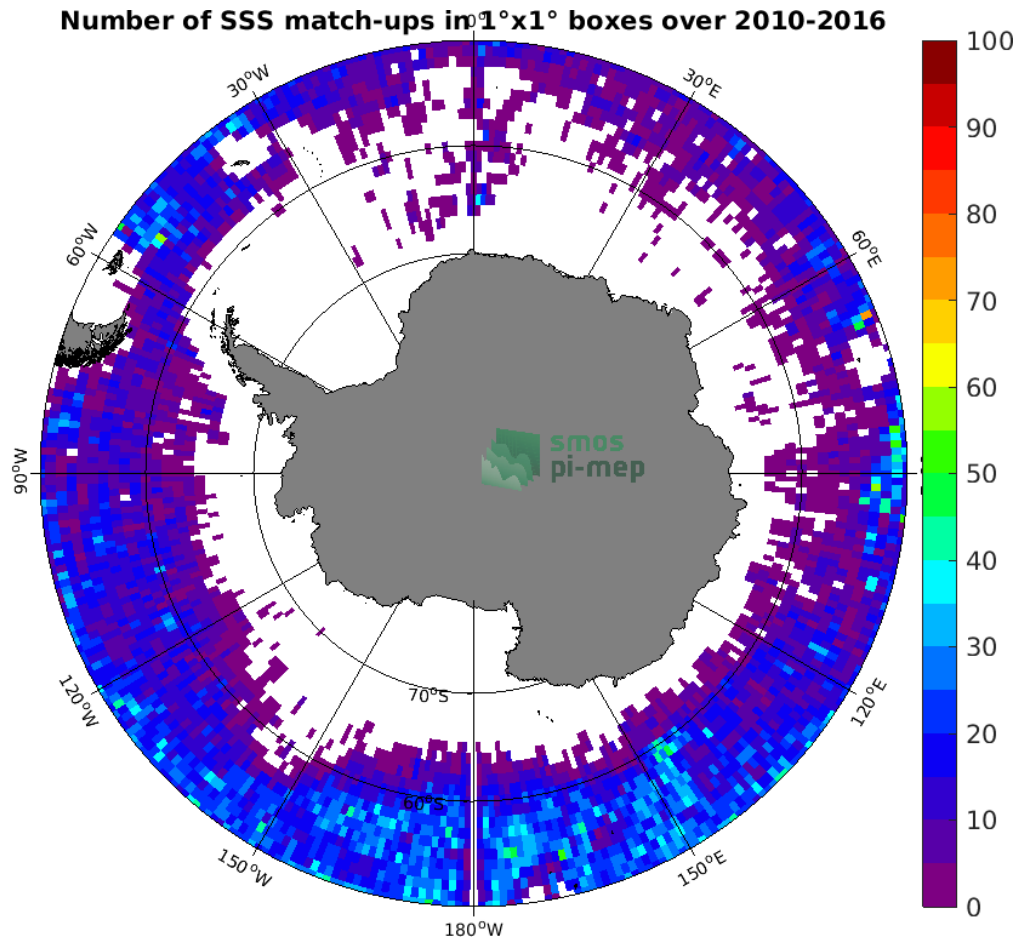
Figure 4: Number of SSS match-ups between Argo SSS and the SMOS SSS L3 v3 Monthly (ICDC) SSS product for the Southern Ocean Pi-MEP region over 1^\circ \times 1^\circ boxes and for the full satellite product period.
