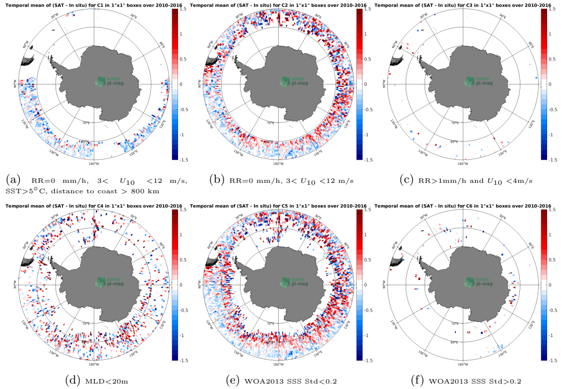
Figure 12: Temporal mean gridded over spatial boxes of size 1^{\circ}\times 1^{\circ} of \Delta\text{SSS} (SMOS SSS L3 v3 Monthly (ICDC) - Argo) for 6 different subdatasets corresponding to: \text{RR}=0 mm/h, 3 < U_{10} < 12 m/s, \text{SST}>5^{\circ}\text{C} , distance to coast > 800 km (a), \text{RR}=0 mm/h, 3 < U_{10} < 12 m/s (b), \text{RR}>1\text{mm/h} and U_{10} < 4\text{m/s} (c), \text{MLD}<20\text{m} (d), \text{WOA2013 SSS Std}<0.2 (e), \text{WOA2013 SSS Std}>0.2 (f).
