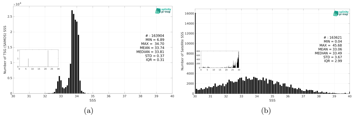
Figure 3: Histograms of SSS from TSG (SAMOS) (a) and SMOS SSS L2Q v331 - With FLAG (CMEMS-CATDS-CPDC) (b) considering all match-up pairs per bins of 0.1 over the Southern Ocean Pi-MEP region and for the full satellite product period.
