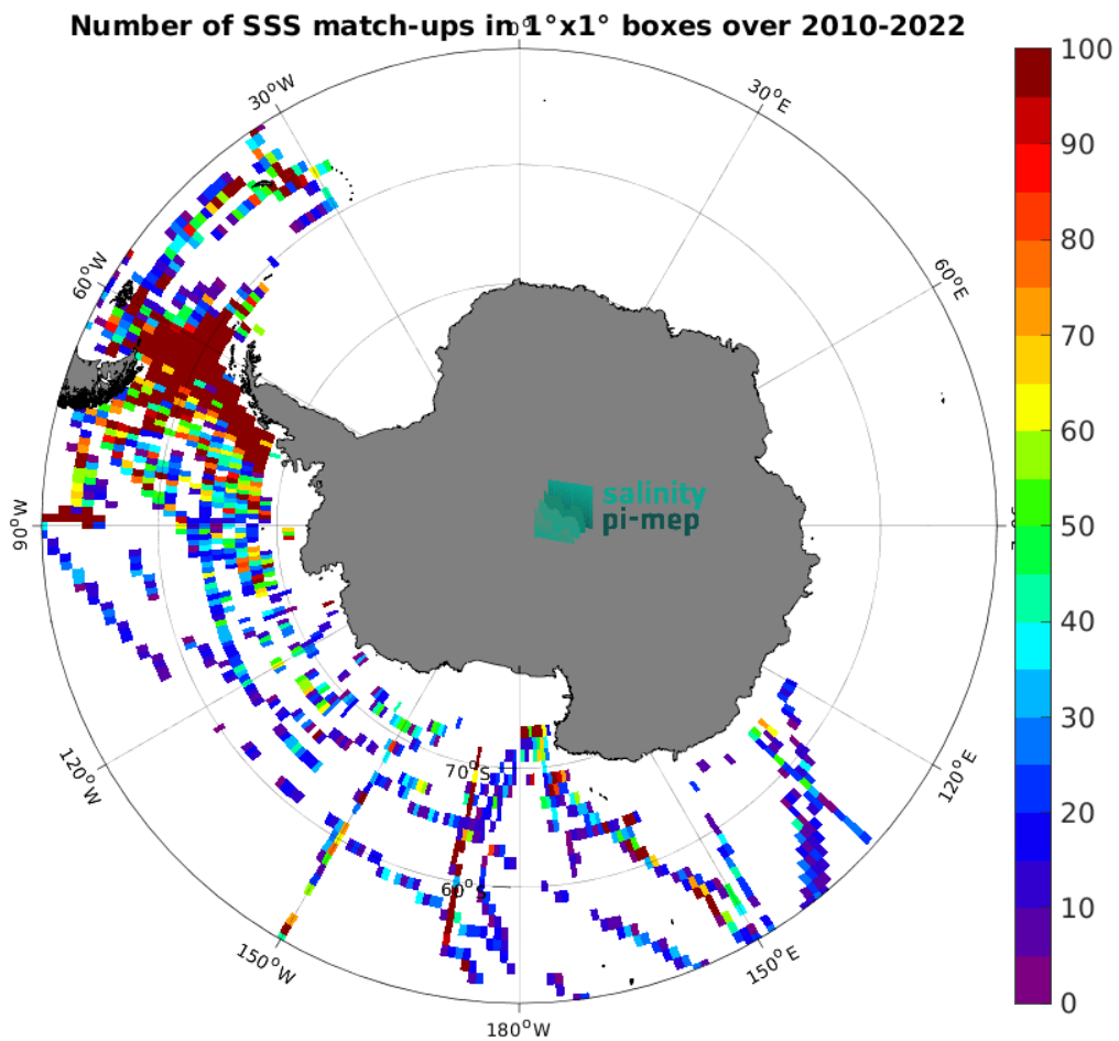
Figure 5: Number of SSS match-ups between TSG (SAMOS) SSS and the SMOS SSS L2Q v331 - With FLAG (CMEMS-CATDS-CPDC) SSS product for the Southern Ocean Pi-MEP region over 1^\circ \times 1^\circ boxes and for the full satellite product period.
