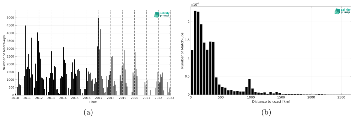
Figure 2: Number of match-ups between TSG (SAMOS) and SMOS SSS L2Q v331 - With FLAG (CMEMS-CATDS-CPDC) SSS as a function of time (a) and as function of the distance to coast (b) over the Southern Ocean Pi-MEP region and for the full satellite product period.
